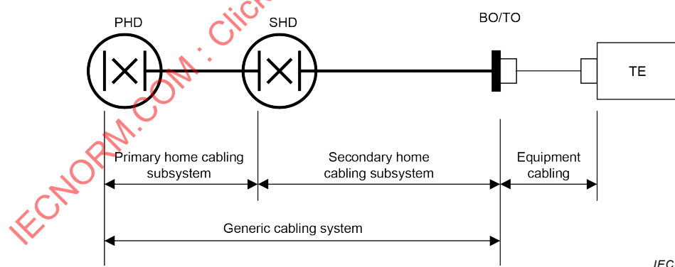
Figure 2 – Structure of the generic cabling system
