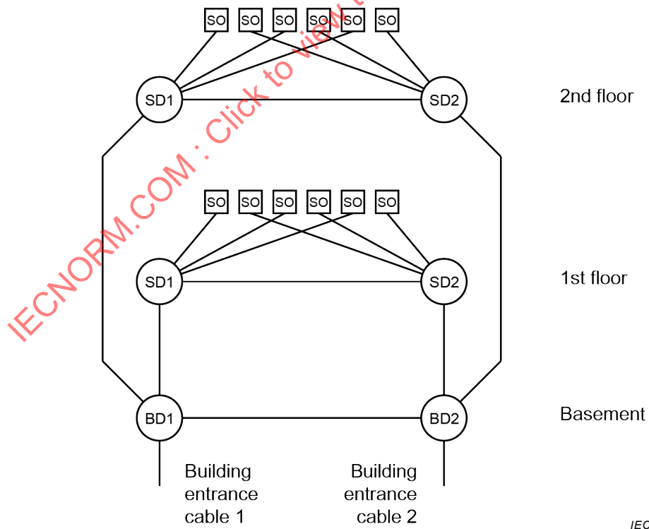
Figure 12 – Connection of functional elements providing redundancy for Type A generic cabling
