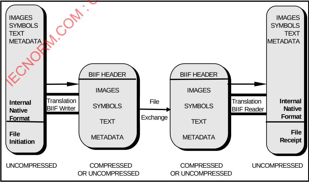
Figure 1 -- Translation process
