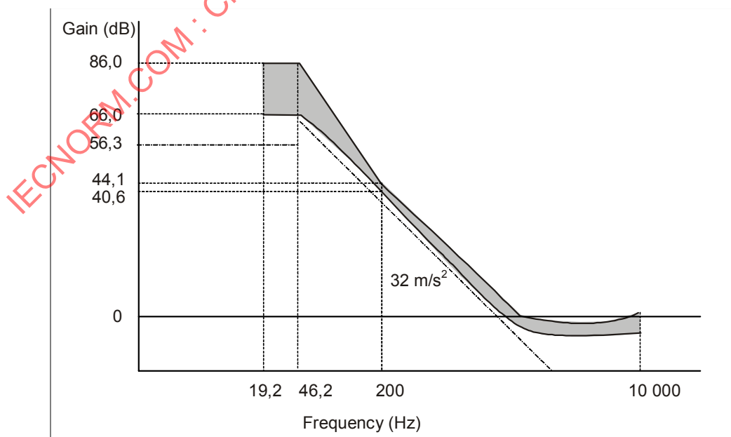
Figure 5 — Reference servo for axial tracking of unrecorded disk
