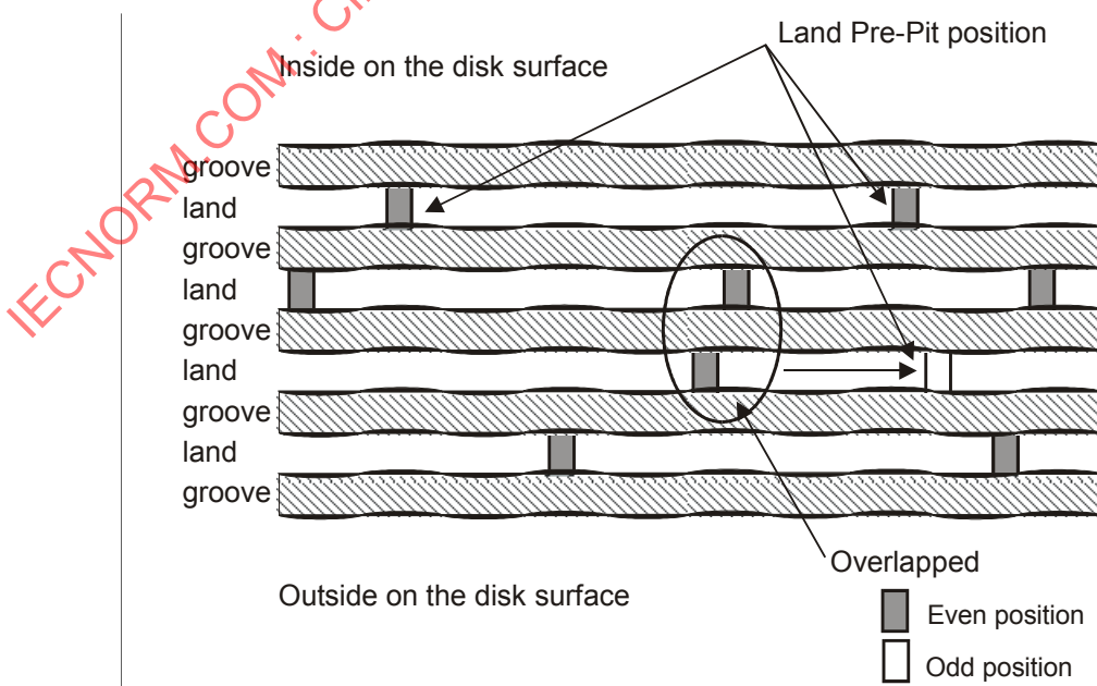
Figure 47 — Layout of land Pre-pit positioning
