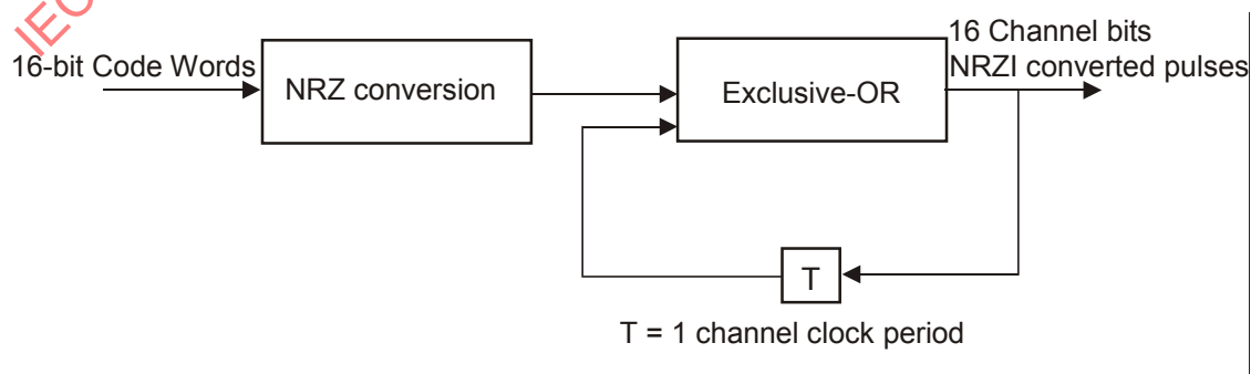
Figure 32 — NRZI conversion
