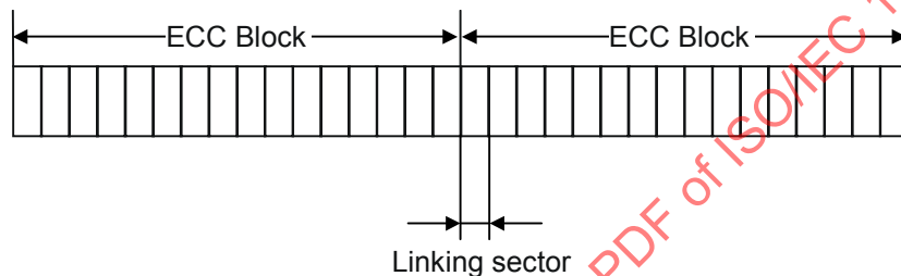
Figure 39 — Structure of ECC Block without Linking Loss Area (Lossless-Link)
