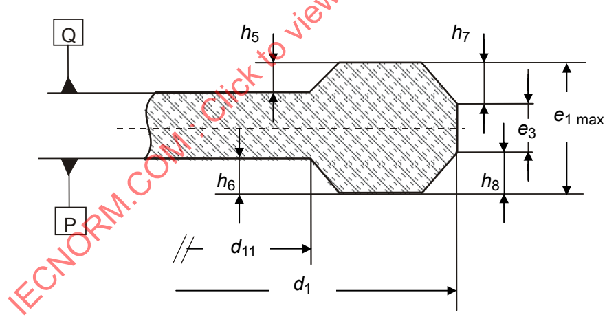
Figure 9 — Rim area
