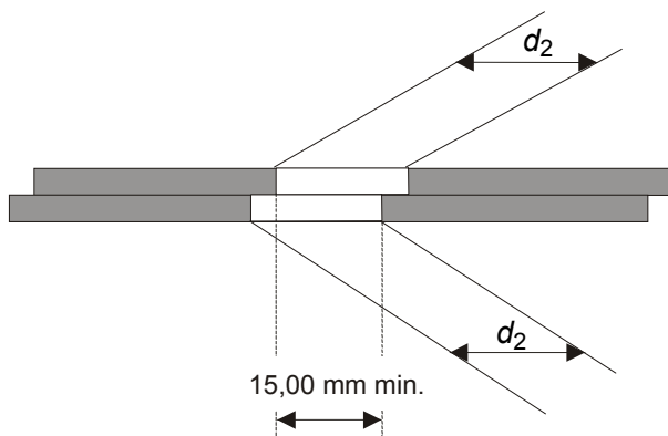
Figure 10 — Hole of the assembled disk
