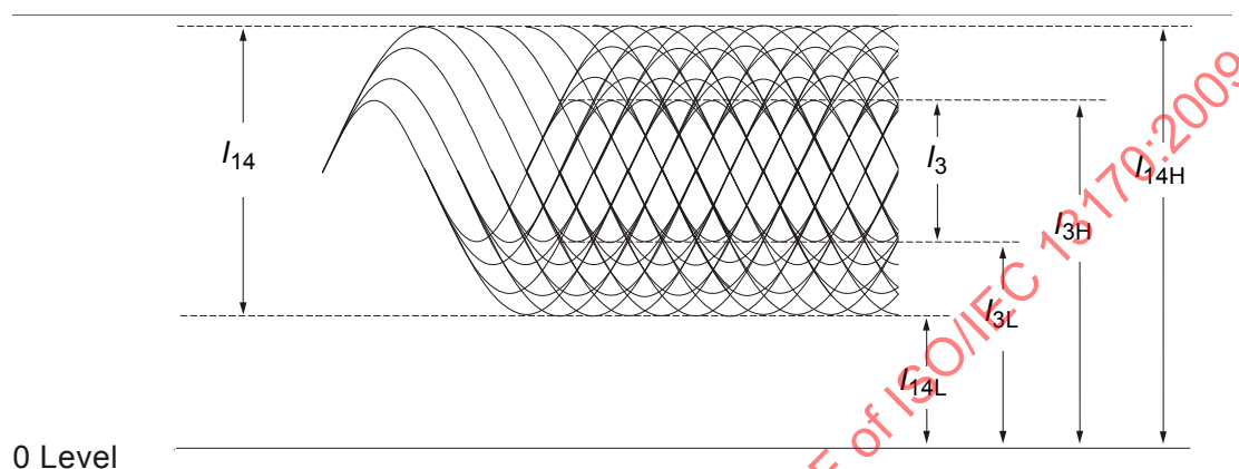
Figure 13 — Modulated amplitude
