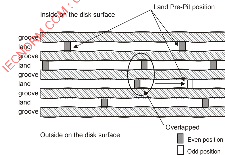
Figure 50 — Layout of land Pre-pit positioning
