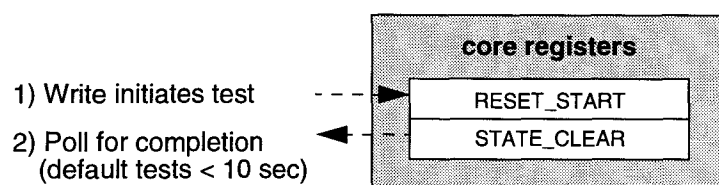
Figure 19—Diagnostic test interface
