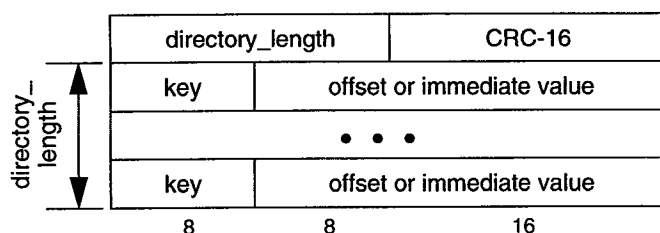
Figure 57—Directory structure
