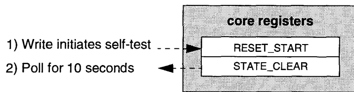
Figure 18—Initialization test interface
