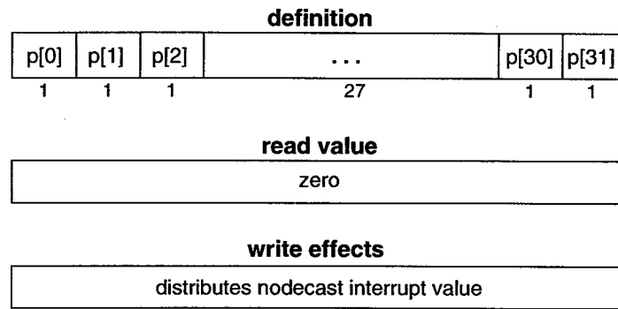
Figure 45—INTERRUPT_TARGET format
