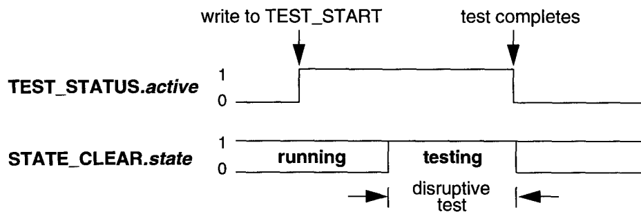
Figure 20—Disruptive test interface
