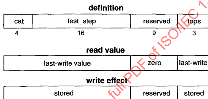
Figure 37—TEST_START format
