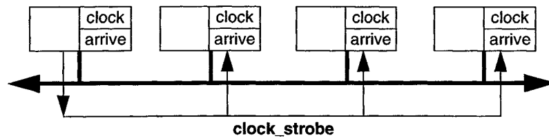
Figure 25—Synchronized node clocks (broadcast backplane mode)
