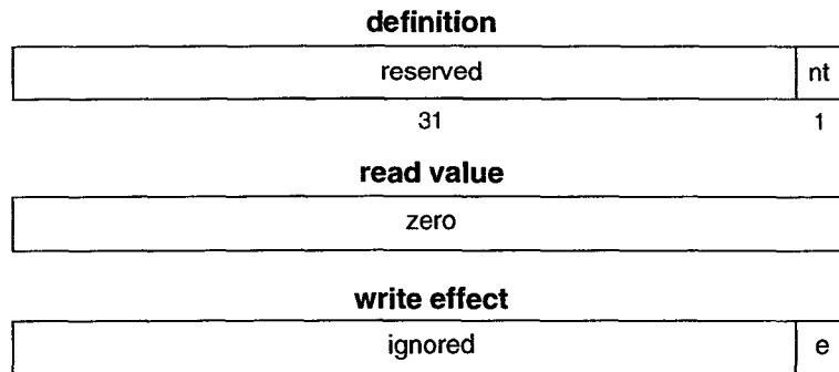
Figure 31 — RESET_START format
