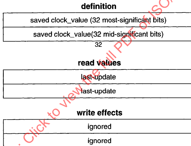
Figure 50—CLOCK_STROBE_ARRIVED formats (read-only)
