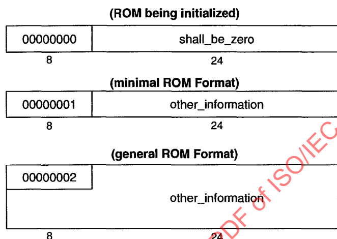
Figure 54—First ROM quadlet
