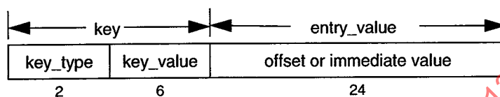
Figure 58—Directory entry format
