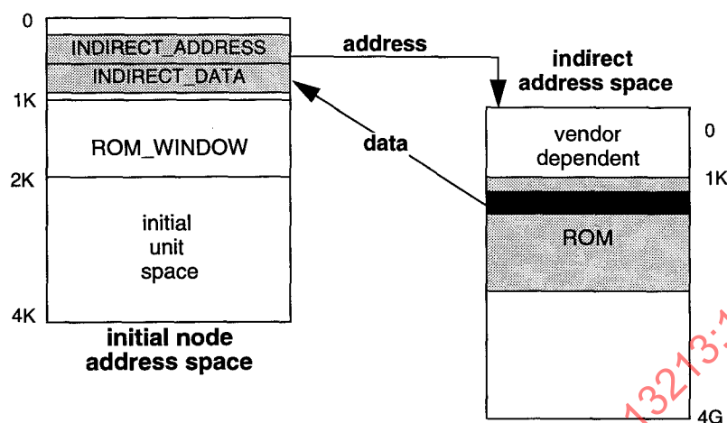
Figure 12—Indirect space mapping (address greater than or equal to 1 kbytes)
