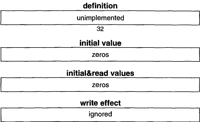
Figure 3—Unimplemented register (hardwired to zero)
