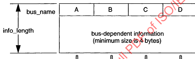
Figure 66—bus_info_block format
