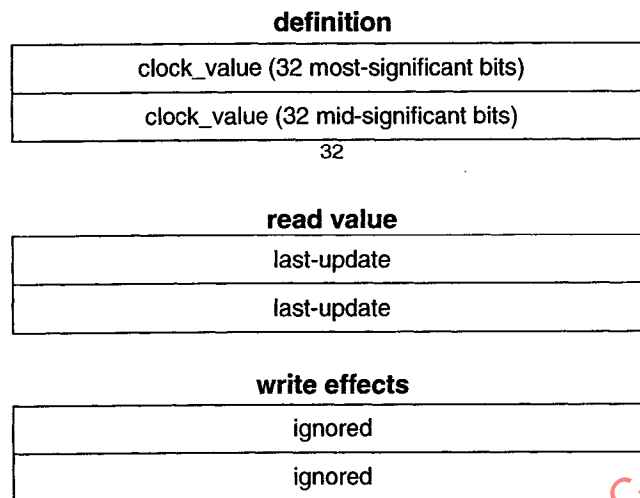
Figure 47—CLOCK_VALUE formats (read-only)
