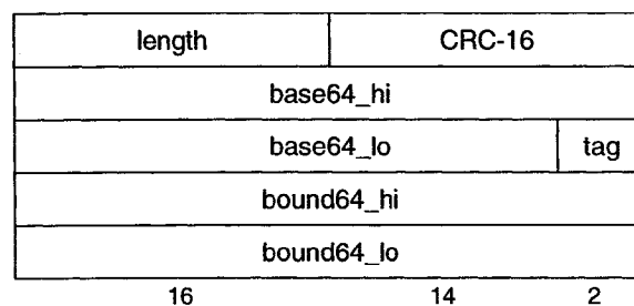
Figure 72—Unit_Locate leaf format
