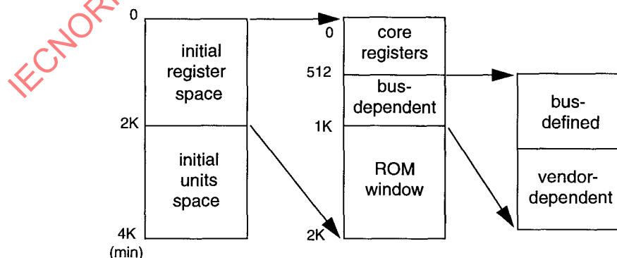
Figure 9—Initial node space components
