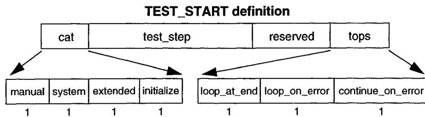
Figure 38— cat and tops formats
