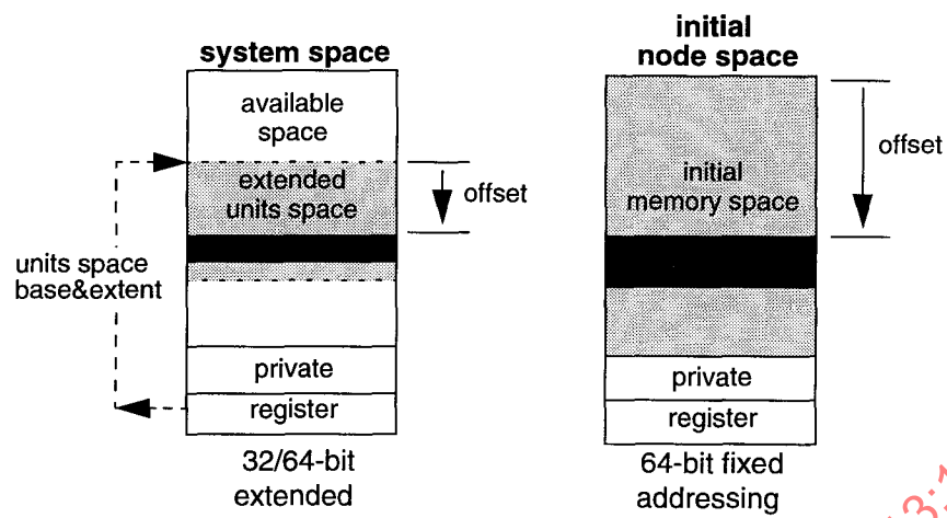
Figure 14—ROM-specified offsets in extended units space
