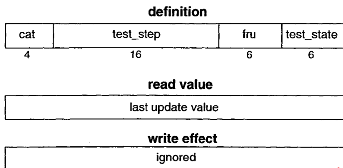
Figure 39—TEST_STATUS format
