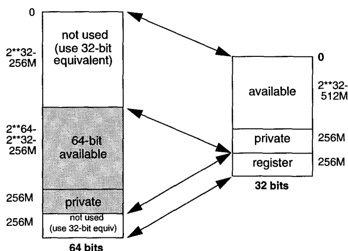
Figure 7—64-bit extended addresses
