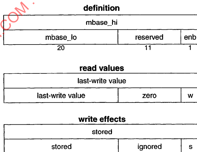
Figure 43—MEMORY_BASE formats
