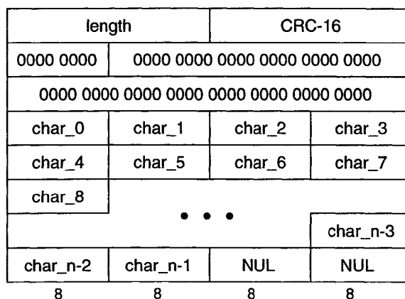
Figure 65—Minimal ASCII textual descriptor leaf format
