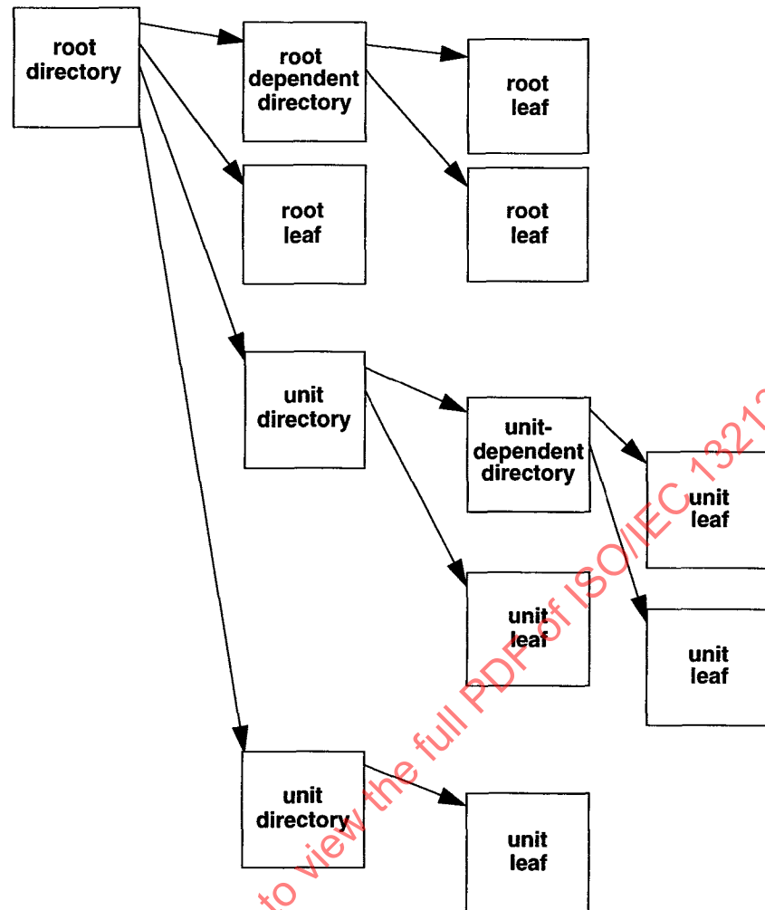
Figure 52—ROM hierarchy
