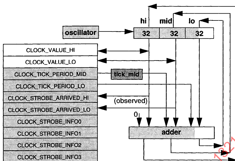
Figure 27—Synchronized clock registers
