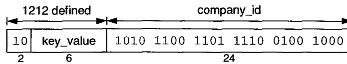
Figure 74—Mapping of company_id bits
