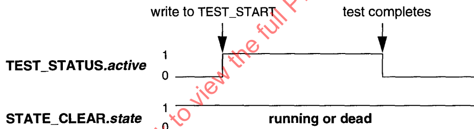
Figure 21—Nondisruptive test interface
