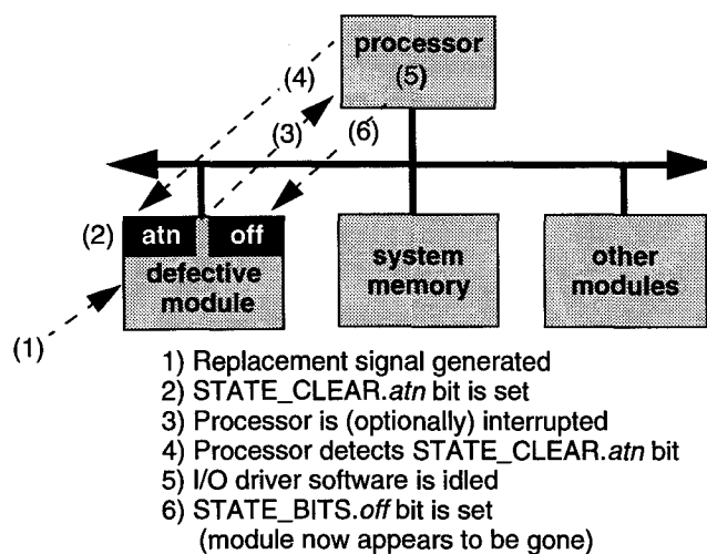
Figure 23—OLR—defective module removal
