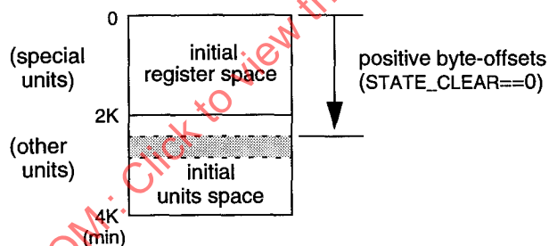
Figure 13—ROM-specified offsets in the initial units space
