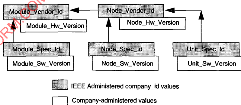
Figure 53—Software identifier hierarchy
