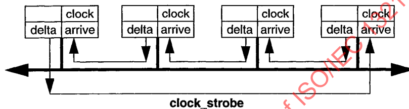
Figure 26—Synchronized clocks (pipelined backplane model)
