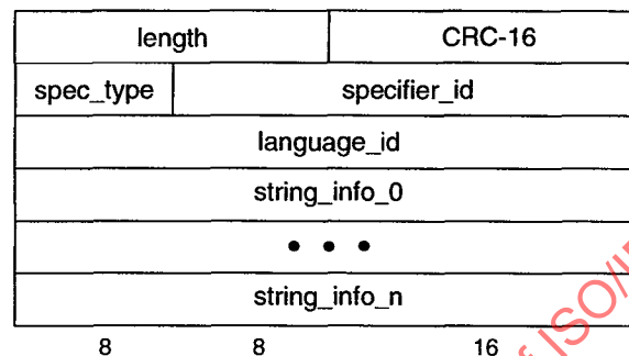
Figure 64—Textual descriptor leaf
