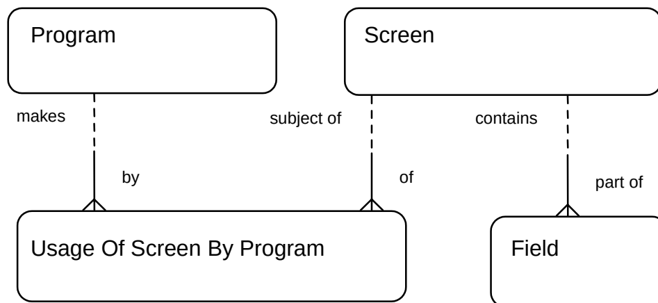
Figure 8: Implementation Data Model
