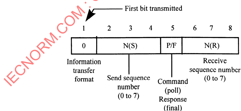
Figure 3a — Information transfer format of control field bits for modulo 8 numbering
