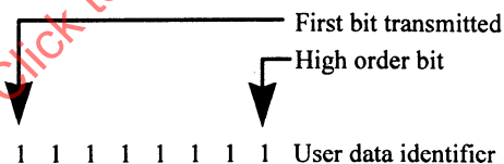
Figure 23 — User data subfield encoding
