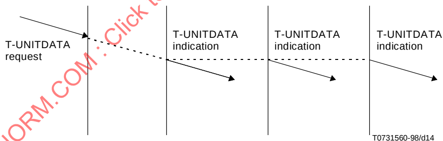
Figure 13 – Sequence of primitives in data transfer using T-UNITDATA primitives
