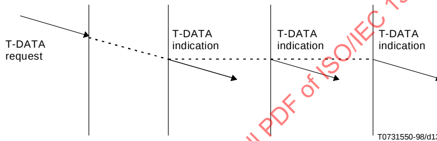
Figure 12 – Sequence of primitives in data transfer using T-DATA primitives
