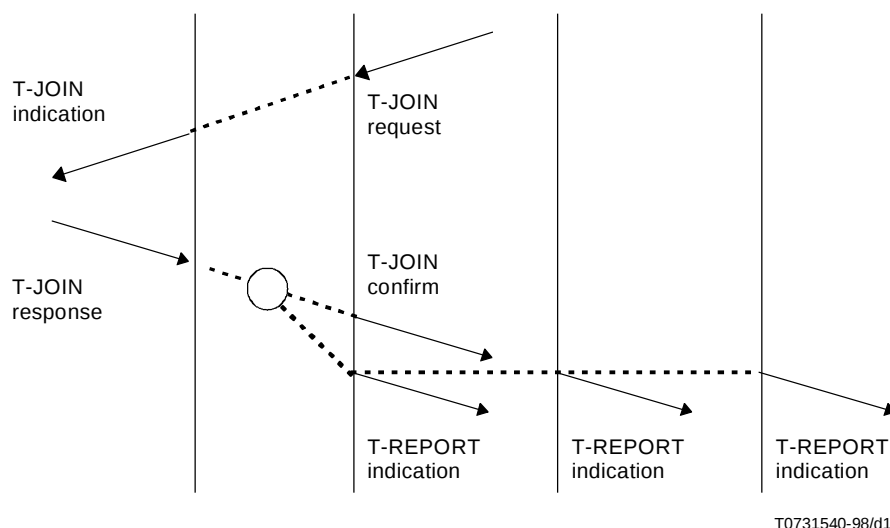
Figure 11 – Sequence of primitives in a successful TC Join by a TS-user in a homogeneous TC or by a receive-only TS-user in a heterogeneous TC
