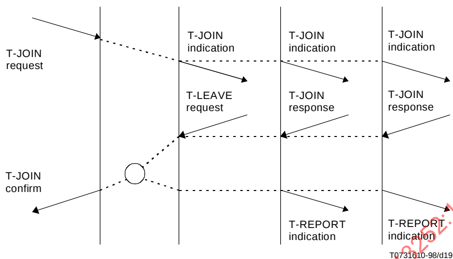
Figure 18 – Sequence of primitives in a successful TC Join with some TS-user rejection(s)
