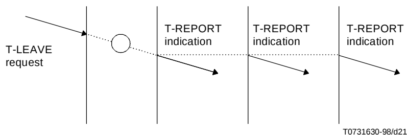
Figure 20 – Sequence of primitives in a TS-user leaving the active TC
