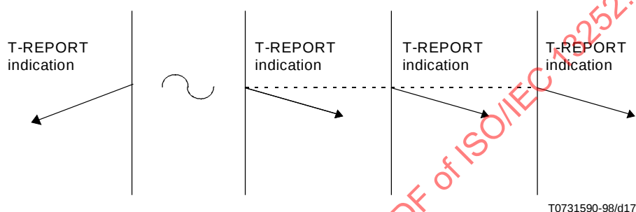
Figure 16 – Sequence of primitives during data transfer when the TS-provider is to give warning or notification
