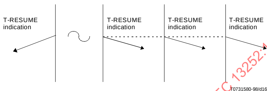
Figure 15 – Sequence of primitives in TS-provider resumption of data transfer
