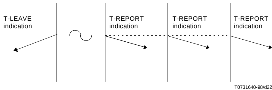
Figure 21 – Sequence of primitives in TS-provider expulsion of TS-user
