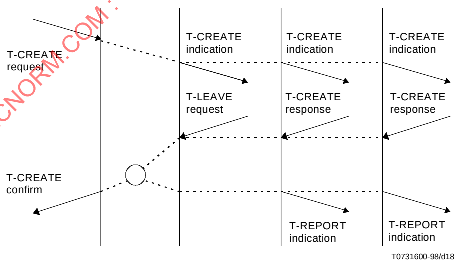
Figure 17 – Sequence of primitives in a successful TC Creation with some TS-user rejection(s)
