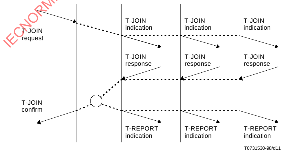
Figure 10 – Sequence of primitives in a successful TC Join by a focal TS-user
