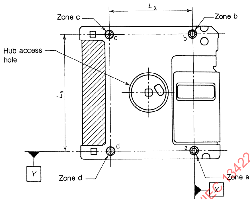
Figure A.1 - Location of the reference zones
