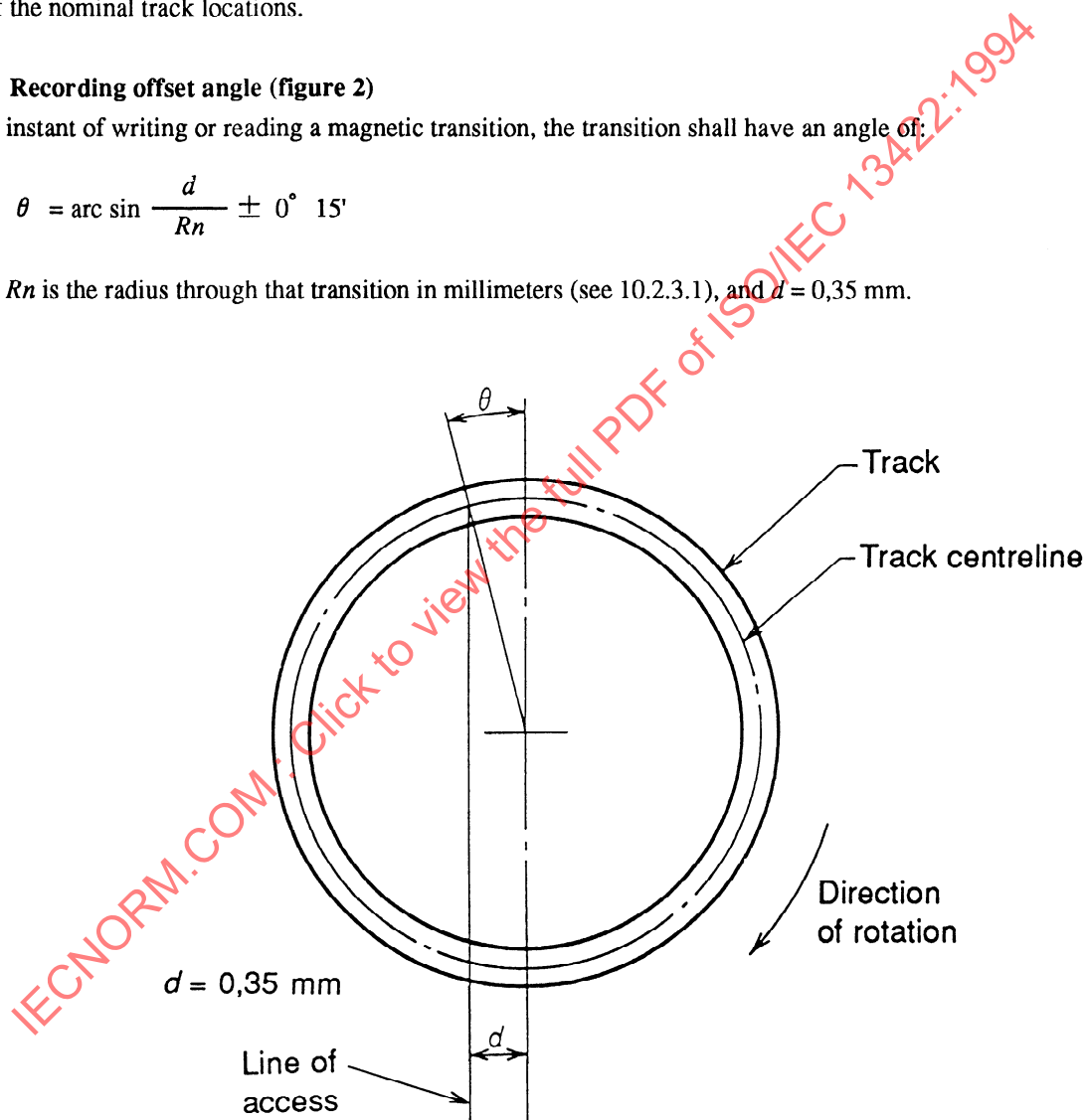
Figure 2 - Recording offset angle
