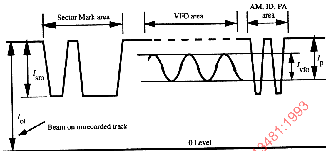
Figure 25b - Signals from Headers in Channel 1
