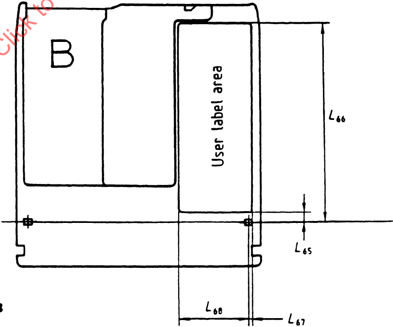
Figure 14.c - User label area on Side B
