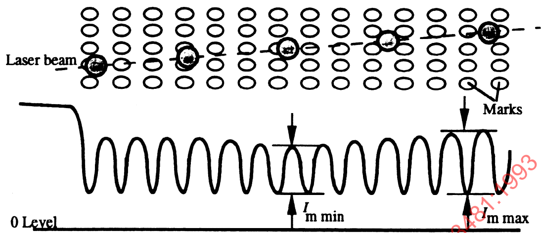
Figure 16 - Path of the laser beam when crossing tracks and the resulting PEP signals
