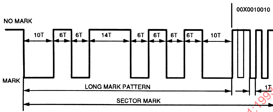
Figure 21 - Sector Mark pattern
