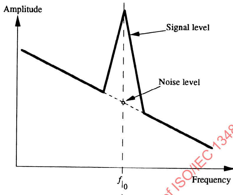
Figure 27 - Amplitude versus frequency for the magneto-optical signal
