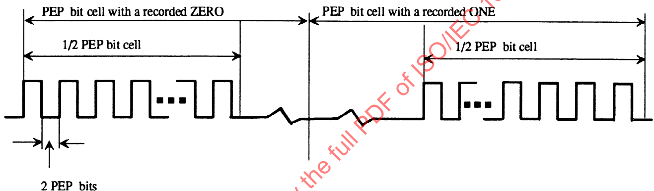
Figure 15 - Example of phase-encoded modulation in the PEP Zone
