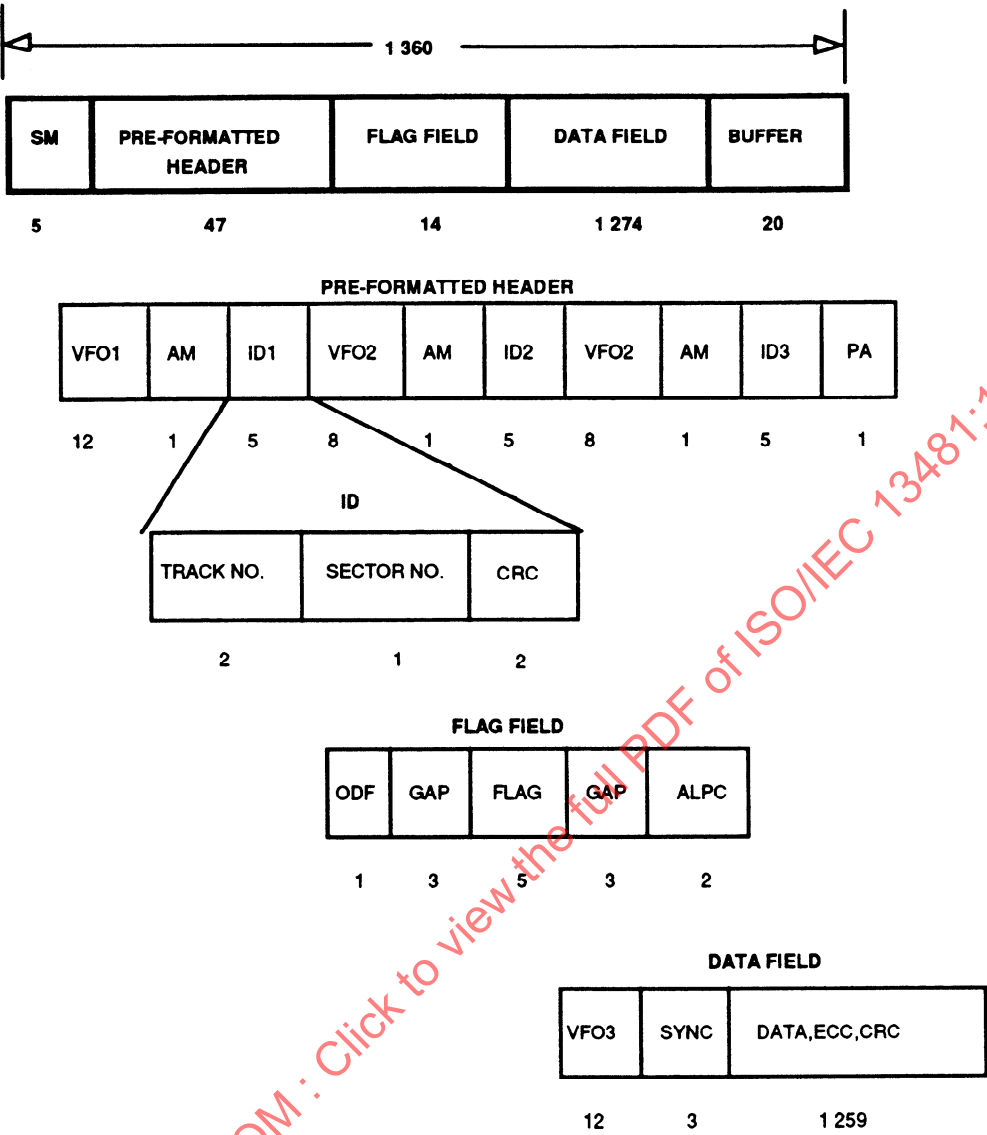
Figure 19 - Sector format for 1 024 user bytes
