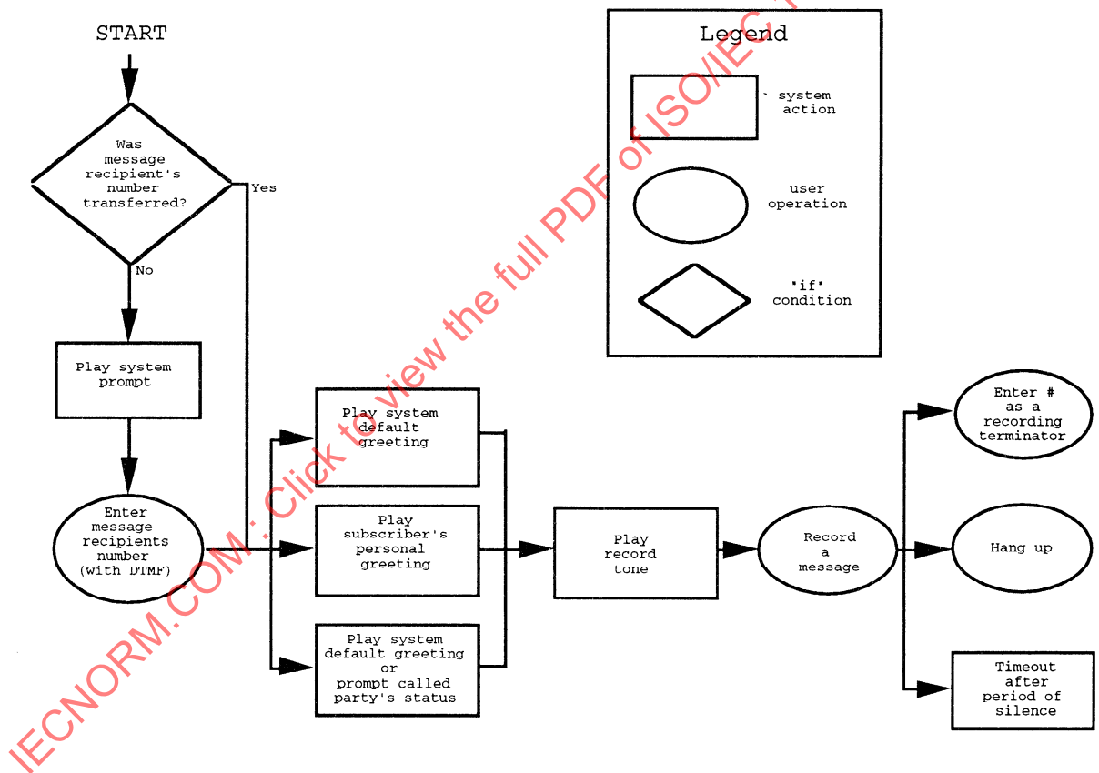
Figure 4 - Sample call flow for call answering
