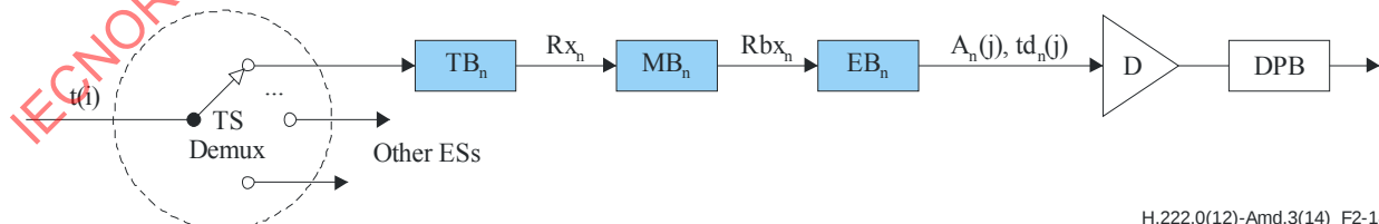
Figure 2-18 – T-STD model extensions for single layer HEVC
