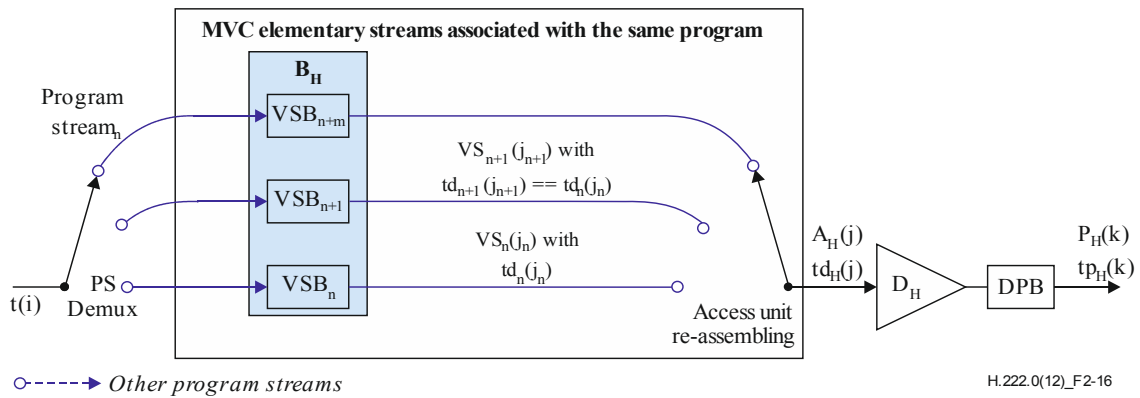
Figure 2-16 – P-STD model extensions for Rec. ITU-T H.264 | ISO/IEC 14496-10 Video with MVC video sub-bitstreams
