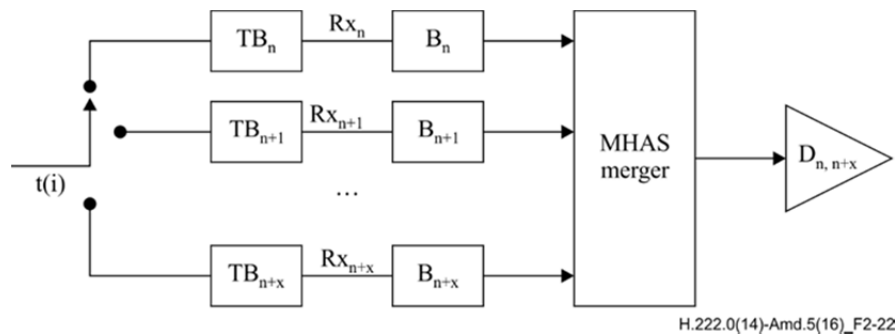
Figure 2-22 – Transport stream system target decoder for multiple audio elementary streams
