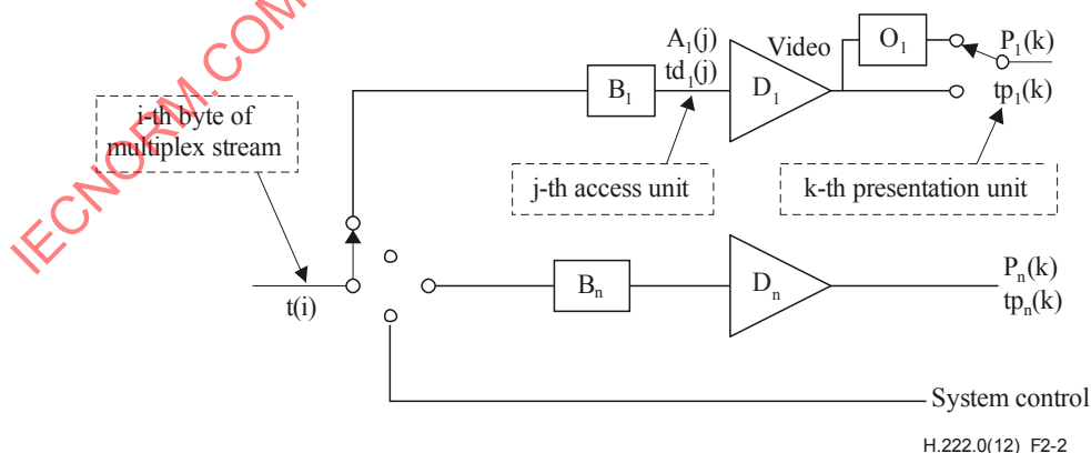
Figure 2-2 – Program stream system target decoder notation
