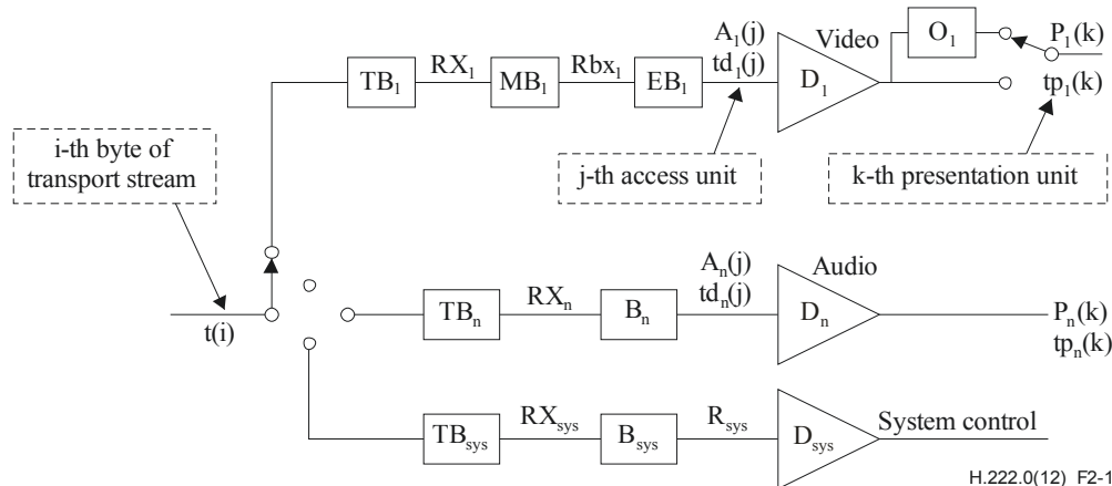
Figure 2-1 – Transport stream system target decoder notation
