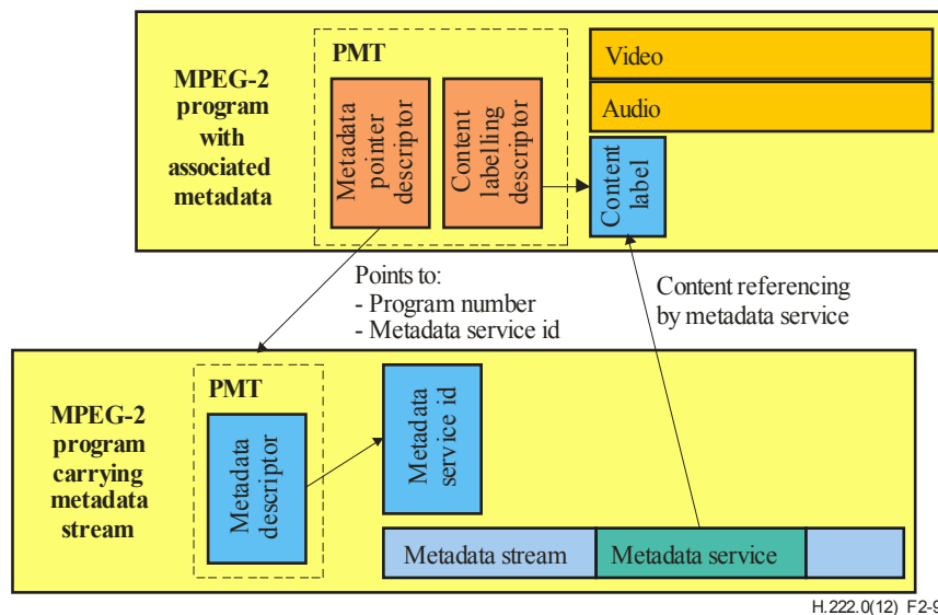
Figure 2-9 – Metadata signalling and referencing
