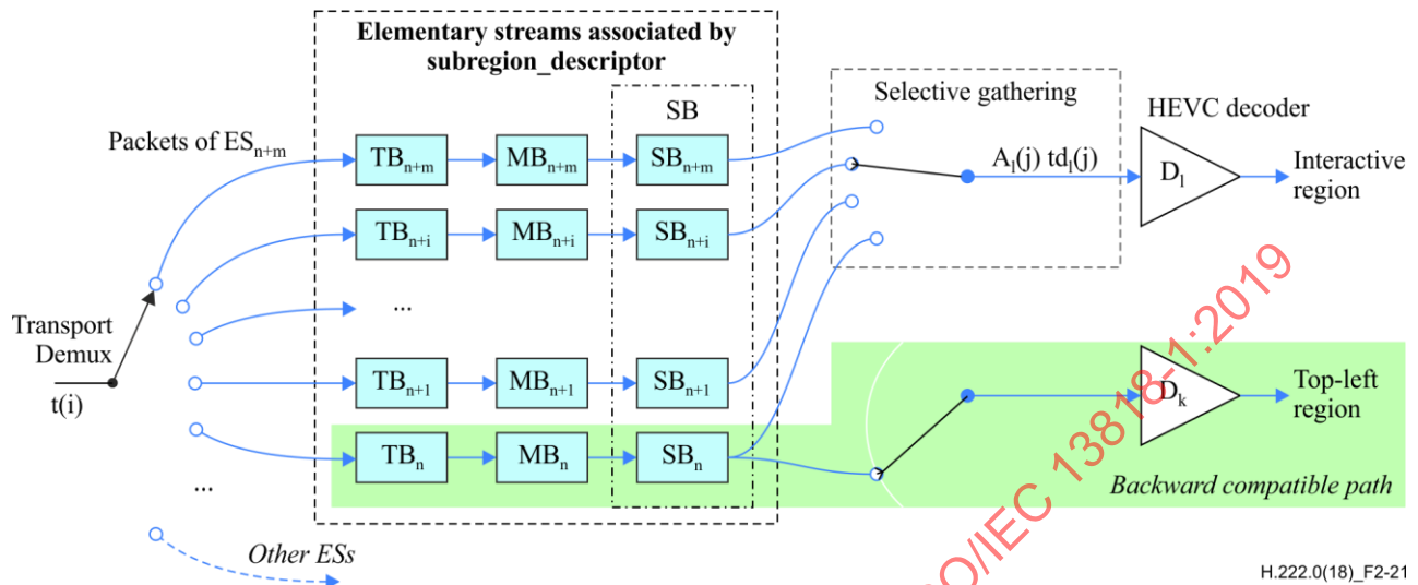
Figure 2-21 – T-STD model extensions for transport of HEVC tiles through individual ESs
