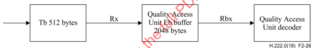
Figure 2-26 – Quality Access Unit decoder processing model
