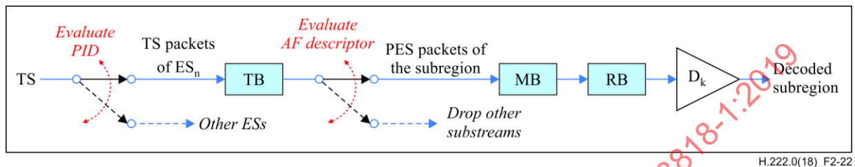
Figure 2-22 – T-STD model extensions for transport of HEVC tiles in a common ES using AF descriptors
