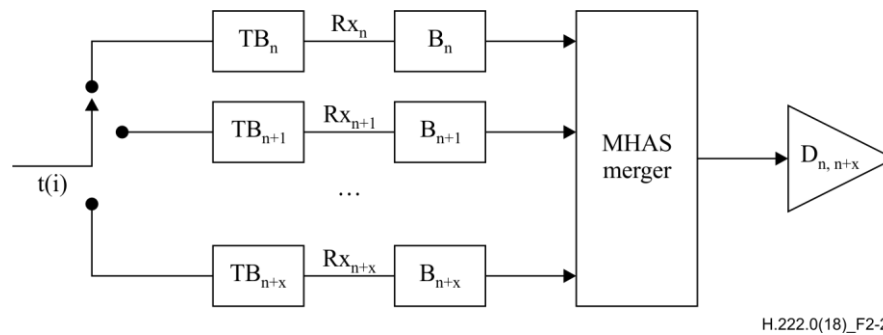
Figure 2-25 – Transport stream system target decoder for multiple audio elementary streams
