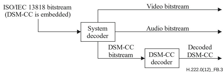
Figure B.3 – DSM-CC bitstream decoded as part of the system bitstream
