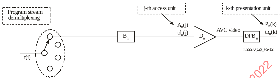
Figure 2-12 – P-STD model extensions for Rec. ITU-T H.264 | ISO/IEC 14496-10 video
