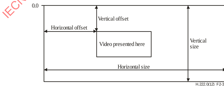
Figure 2-3 – Target background grid descriptor display area
