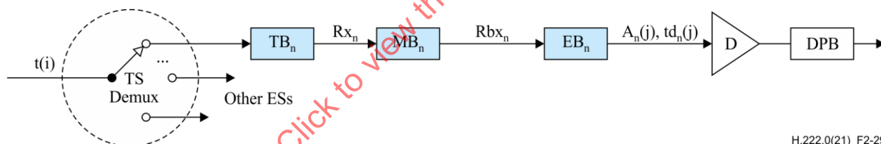
Figure 2-29 – T-STD model extensions for single layer EVC
