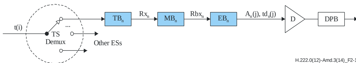
Figure 2-18 – T-STD model extensions for single layer HEVC
