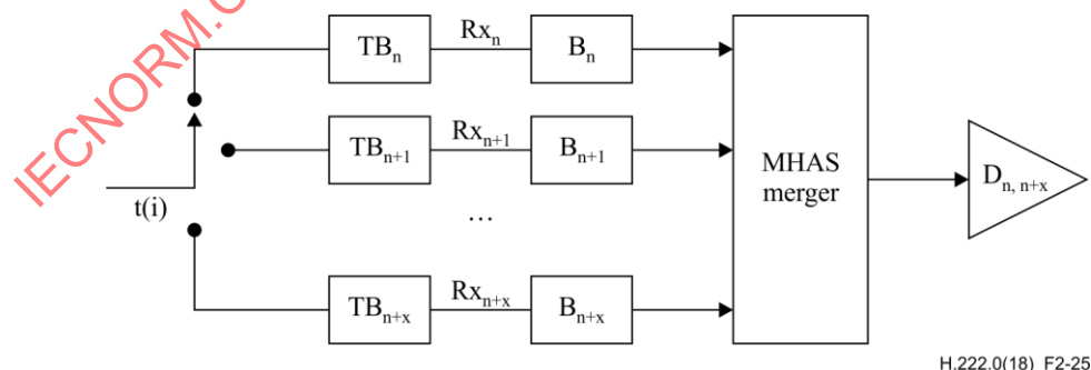
Figure 2-25 – Transport stream system target decoder for multiple audio elementary streams
