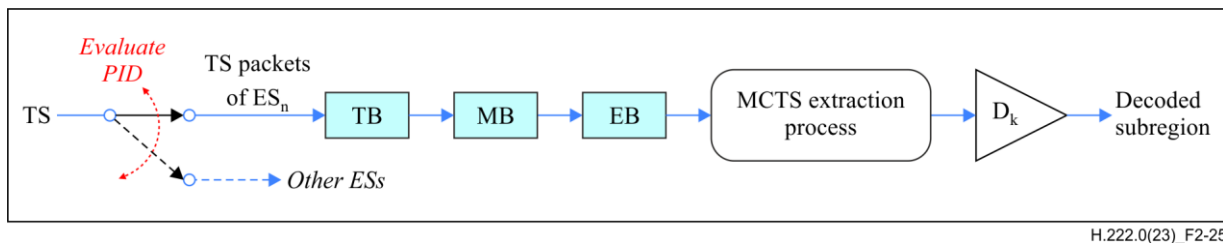
Figure 2-25 – T-STD model extension for transport of HEVC tiles in a common ES ignoring AF descriptors
