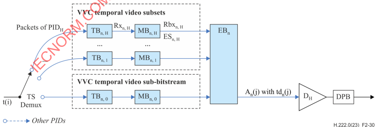
Figure 2-30 – T-STD model extensions for layered transport of VVC temporal video subsets
