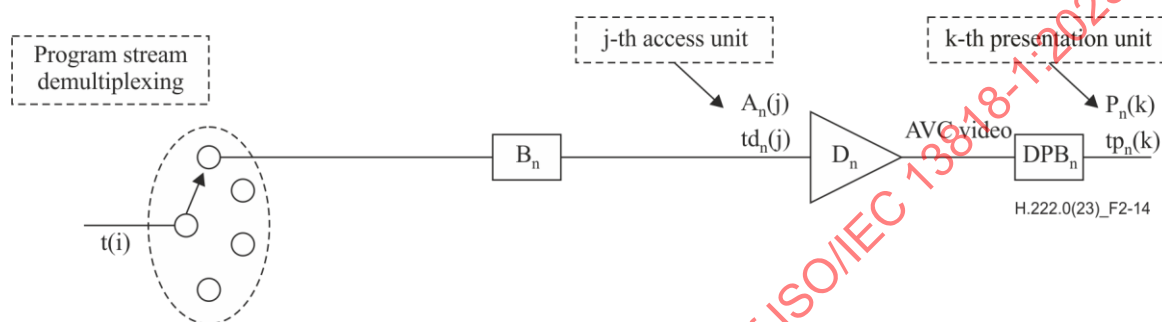
Figure 2-14 – P-STD model extensions for Rec. ITU-T H.264 | ISO/IEC 14496-10 video
