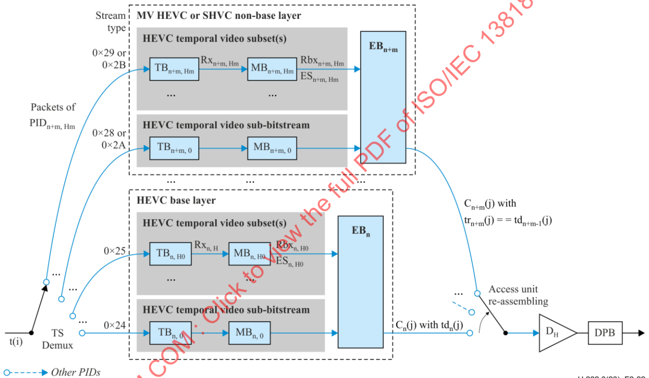
Figure 2-22 – T-STD model extensions for bitstream-partition-specific CPB operation
