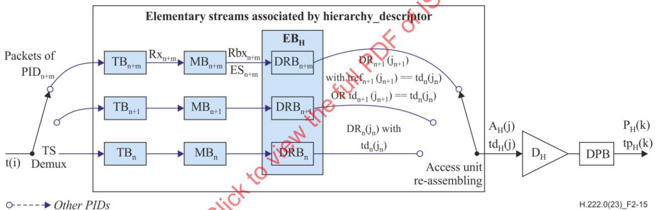
Figure 2-15 – T-STD model extensions for Rec. ITU-T H.264 | ISO/IEC 14496-10 video with scalable video sub-bitstreams
