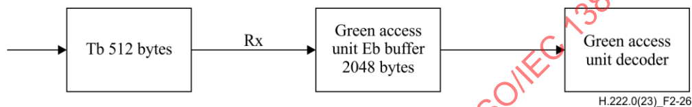
Figure 2-26 – T-STD model extension for green access units
