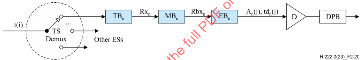
Figure 2-20 – T-STD model extensions for single layer HEVC
