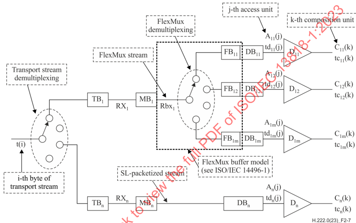
Figure 2-7 – T-STD model for ISO/IEC 14496 content
