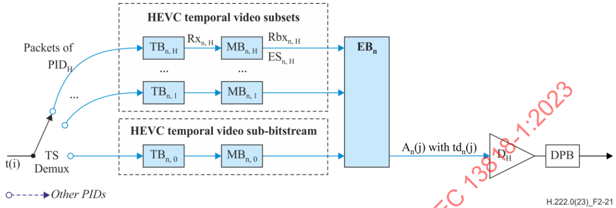
Figure 2-21 – T-STD model extensions for layered transport of HEVC temporal video subsets
