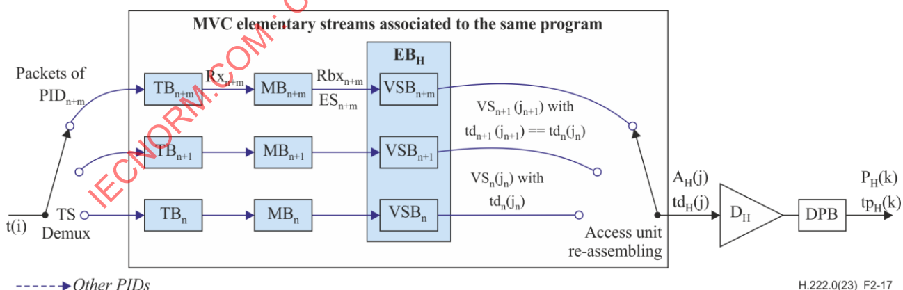
Figure 2-17 – T-STD model extensions for Rec. ITU-T H.264 | ISO/IEC 14496-10 Video with MVC video sub-bitstreams
