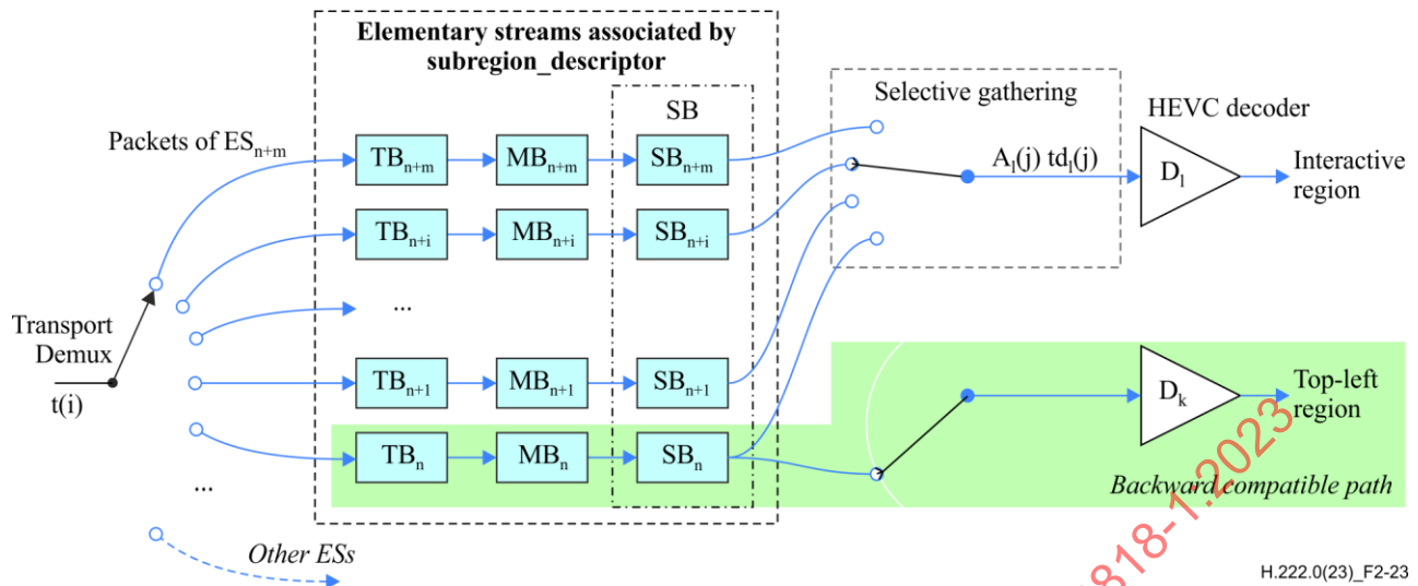
Figure 2-23 – T-STD model extensions for transport of HEVC tiles through individual ESs
