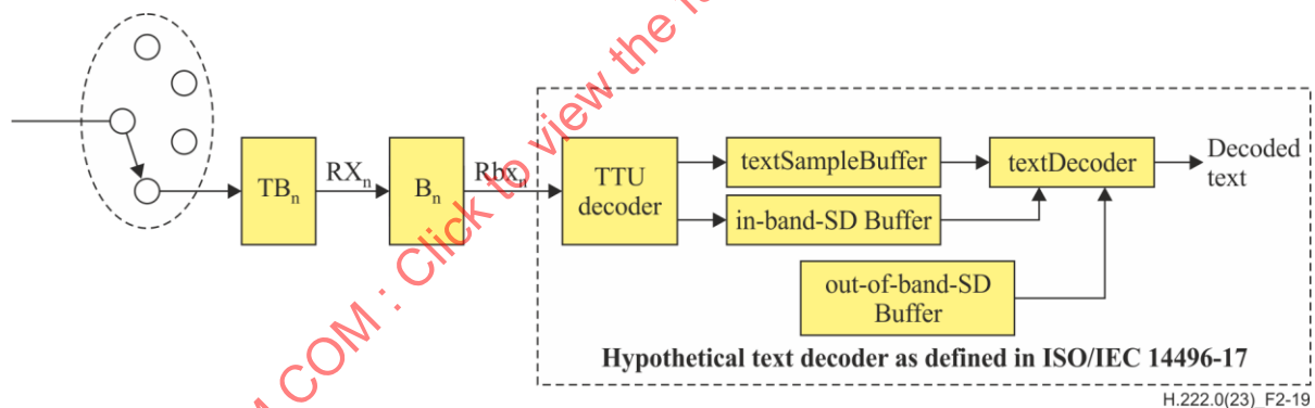
Figure 2-19 – T-STD model extensions for ISO/IEC 14496-17 text streams
