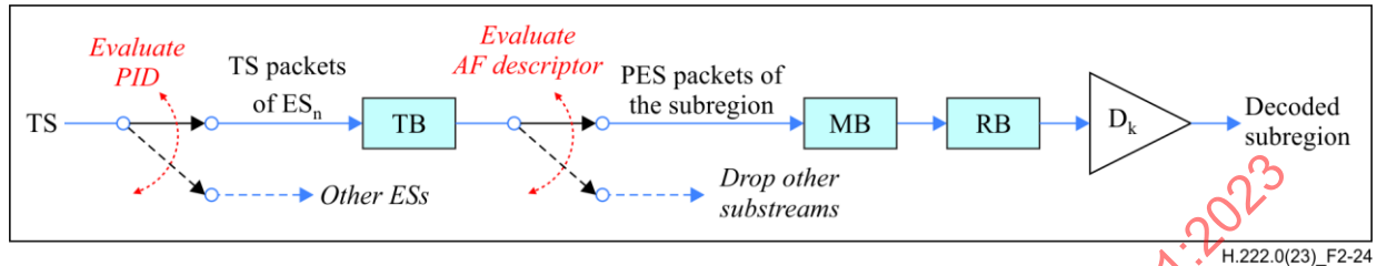
Figure 2-24 – T-STD model extensions for transport of HEVC tiles in a common ES using AF descriptors
