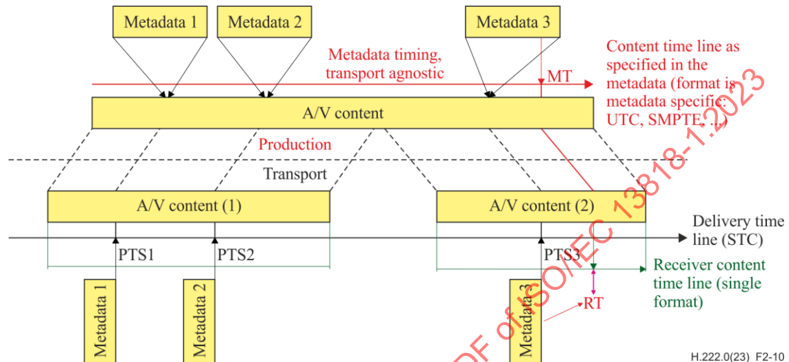
Figure 2-10 – Delivery of metadata in PES packets
