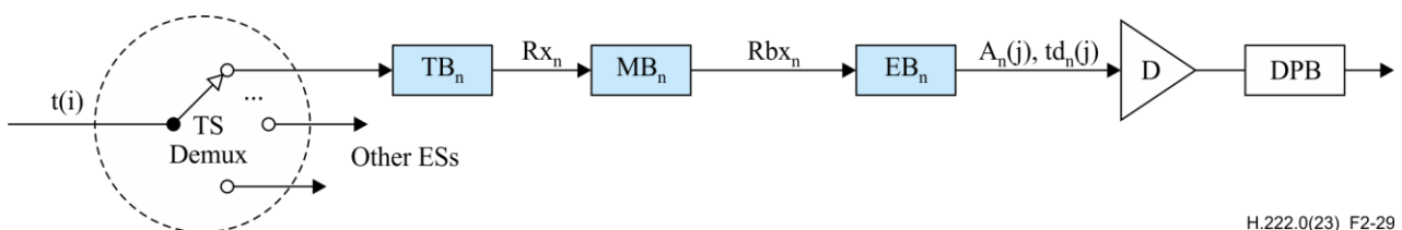
Figure 2-29 – T-STD model extensions for single layer VVC
