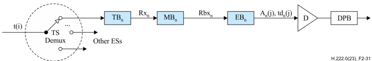
Figure 2-31 – T-STD model extensions for single layer EVC
