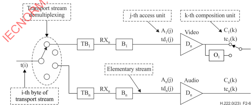
Figure 2-6 – T-STD model extensions for individual ISO/IEC 14496 elementary streams
