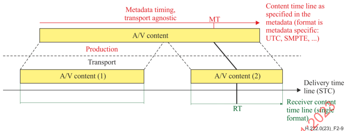
Figure 2-9 – Timing model for delivery of content and metadata
