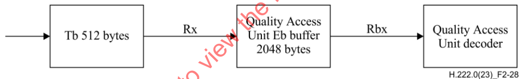
Figure 2-28 – Quality Access Unit decoder processing model
