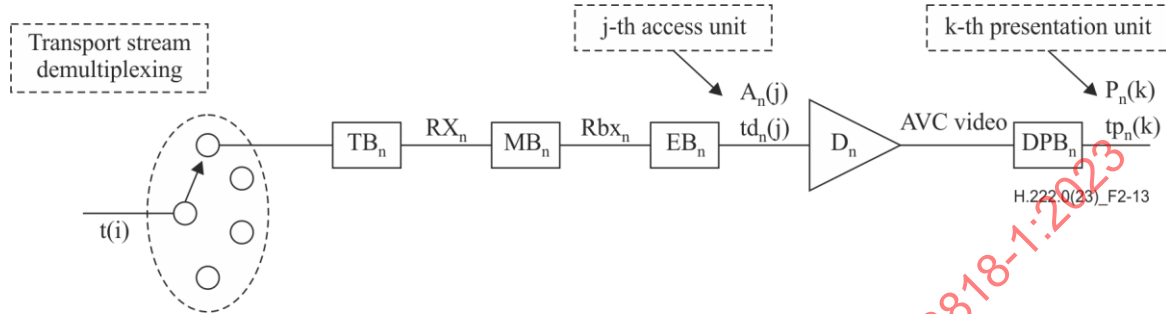
Figure 2-13 – T-STD model extensions for Rec. ITU-T H.264 | ISO/IEC 14496-10 video
