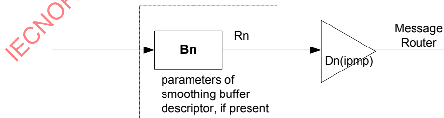
Figure 4 — IPMP Stream Decoder Model in Program Stream
