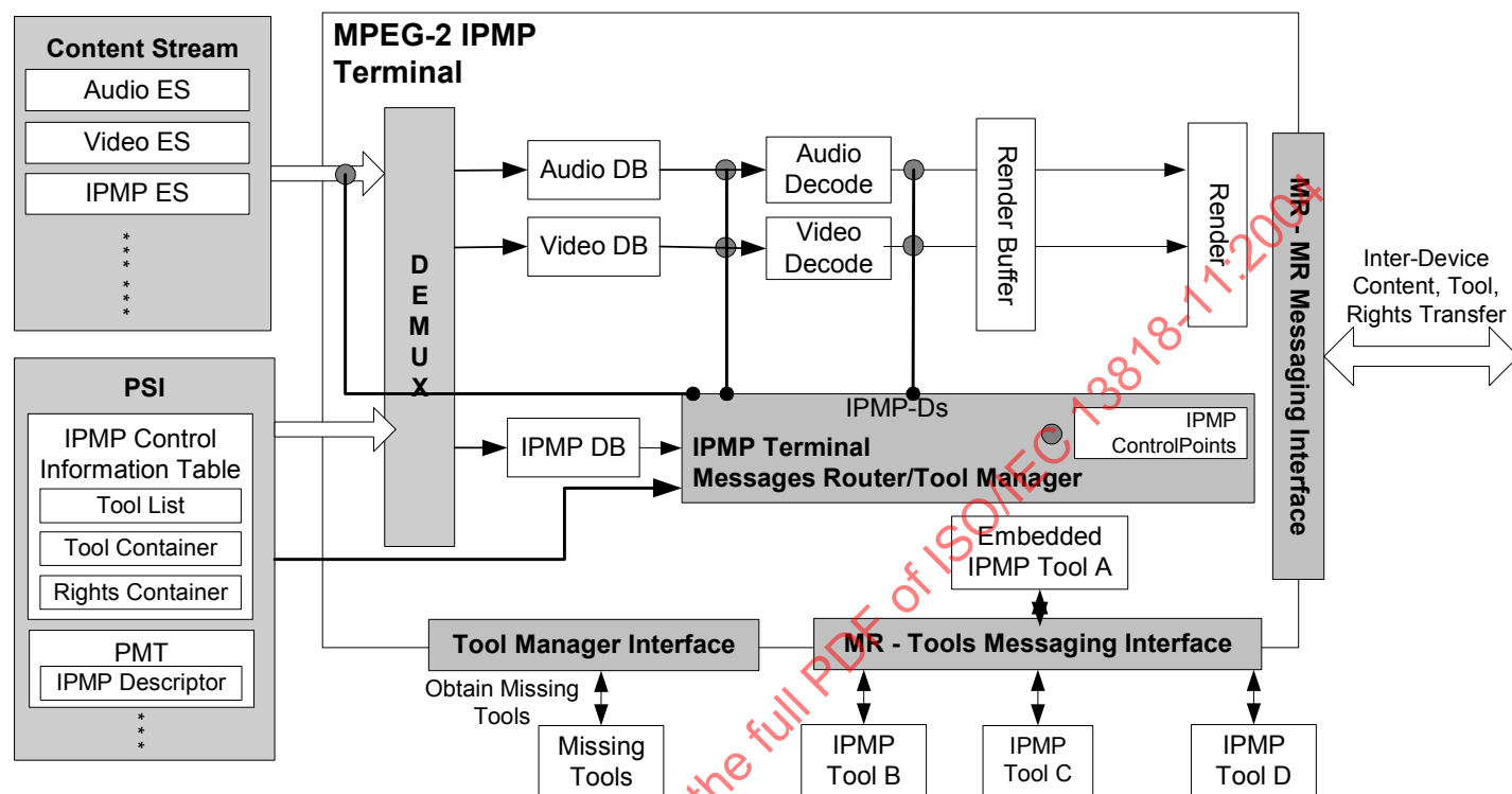
Figure 1 — MPEG-2 IPMP Architecture
