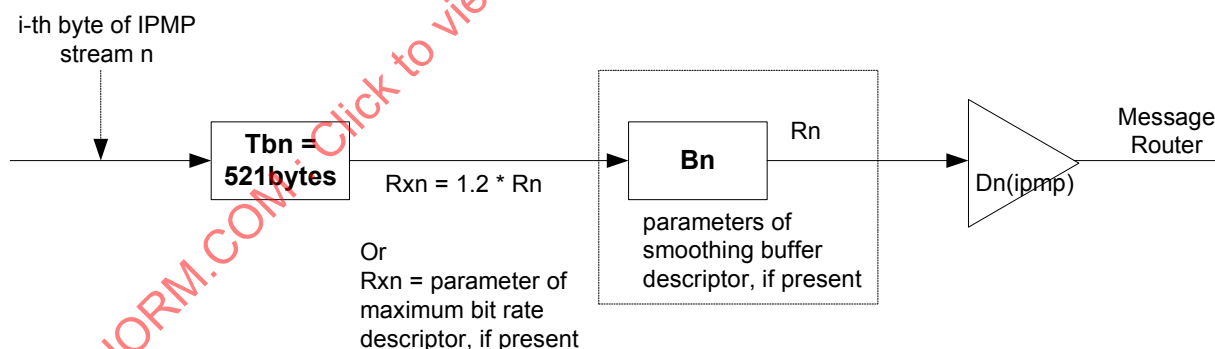
Figure 3 — IPMP Stream Decoder Model in Transport Stream
