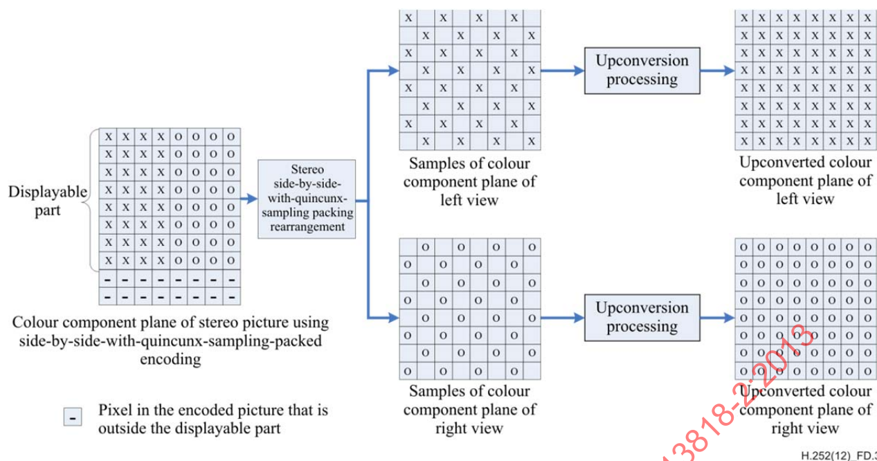
Figure D.3 – Rearrangement and hypothetical upconversion of "stereo side-by-side with quincunx sampling" arrangement views to convert to the full resolution of the displayable part of the encoded picture
