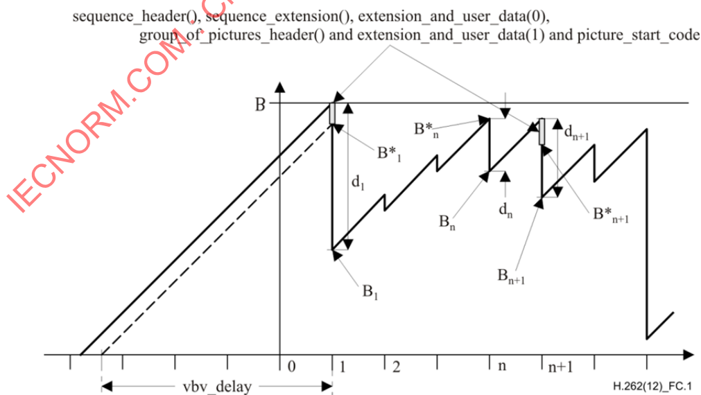
Figure C.1 – VBV buffer occupancy – Constant bit rate operation
