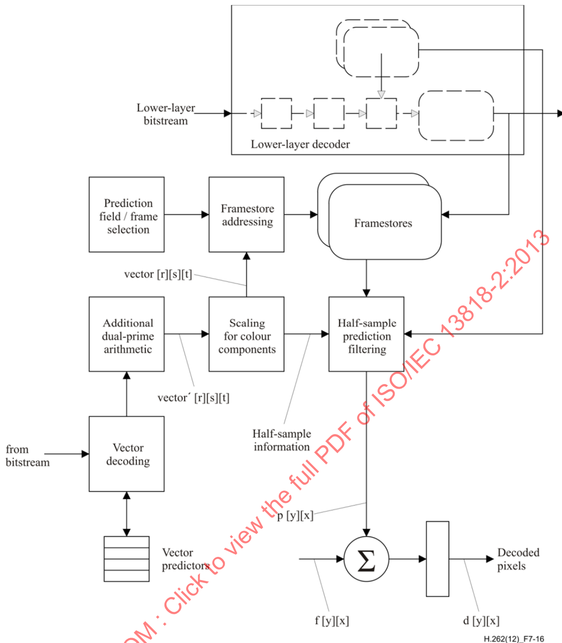
Figure 7-16 – Simplified motion compensation process for the enhancement layer using temporal scalability
