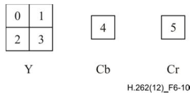
Figure 6-10 – 4:2:0 Macroblock structure
