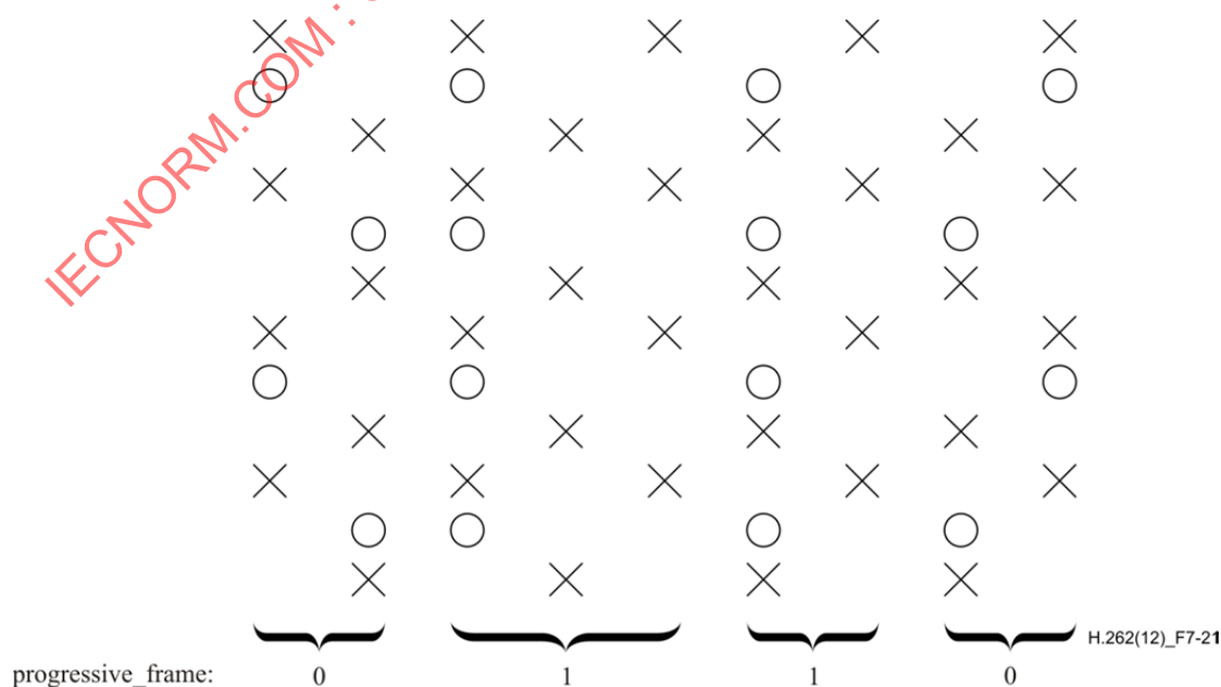
Figure 7-21 – progressive_sequence == 0 with 4:2:0 chrominance
