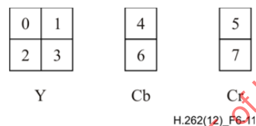
Figure 6-11 – 4:2:2 Macroblock structure
