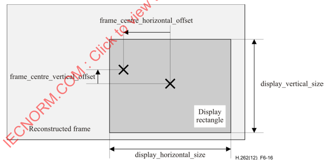
Figure 6-18 – Frame centre offset parameters
