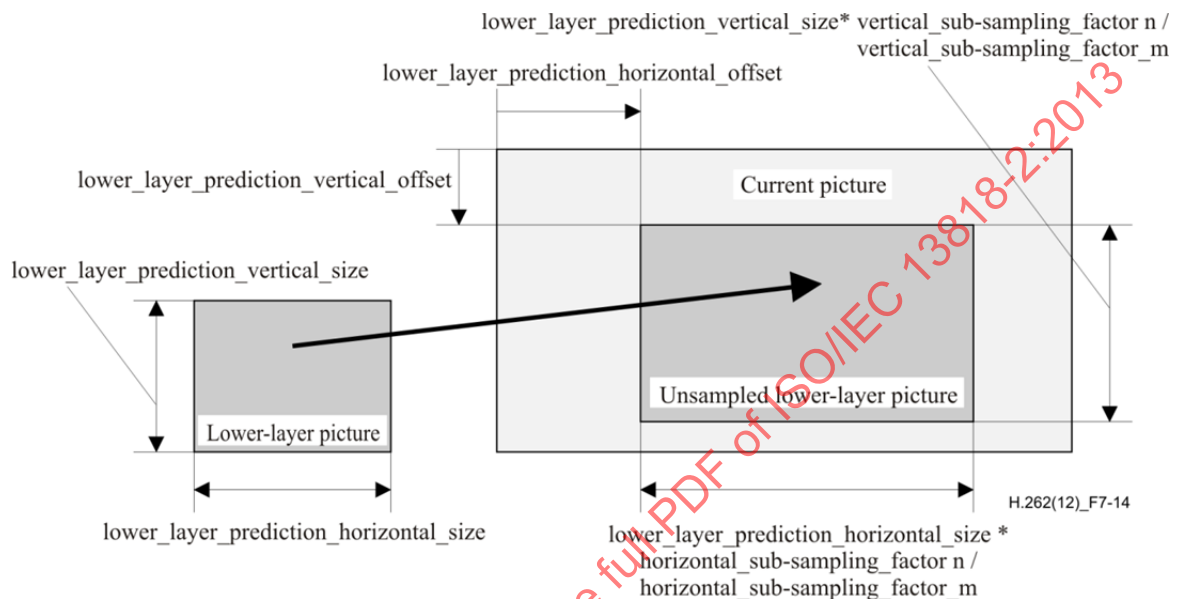
Figure 7-14 – Formation of the "spatial" prediction by interpolation of the lower-layer picture
