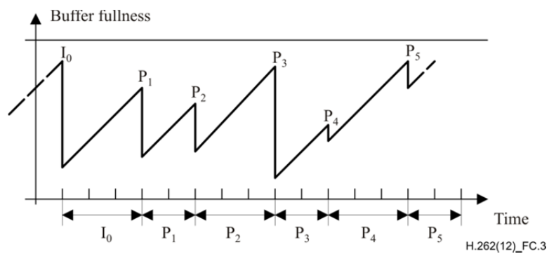
Figure C.3 – Example VBV without B-pictures
