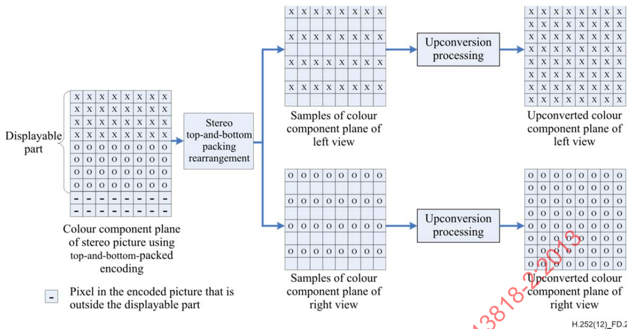
Figure D.2 – Rearrangement and hypothetical upconversion of "stereo top-and-bottom" arrangement views to convert to the full resolution of the displayable part of the encoded picture
