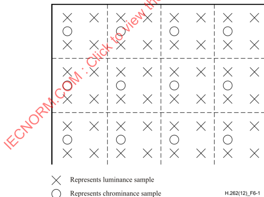
Figure 6-1 – The position of luminance and chrominance samples – 4:2:0 data
