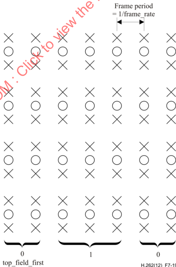
Figure 7-19 – progressive_sequence == '1'; repeat_first_field == '1'
