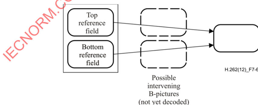
Figure 7-6 – Prediction of the first field or prediction in a frame picture
