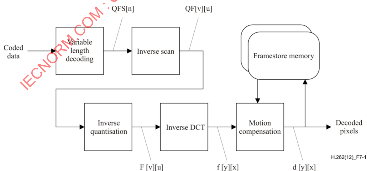
Figure 7-1 – Simplified video decoding process
