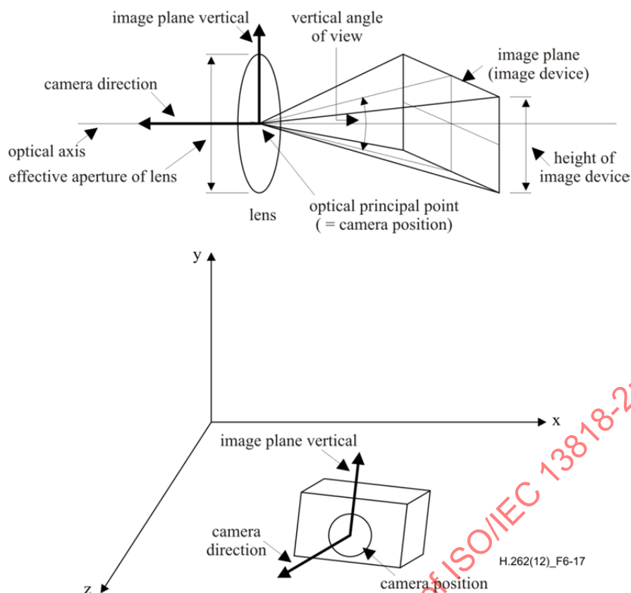
Figure 6-19 – Camera parameters
