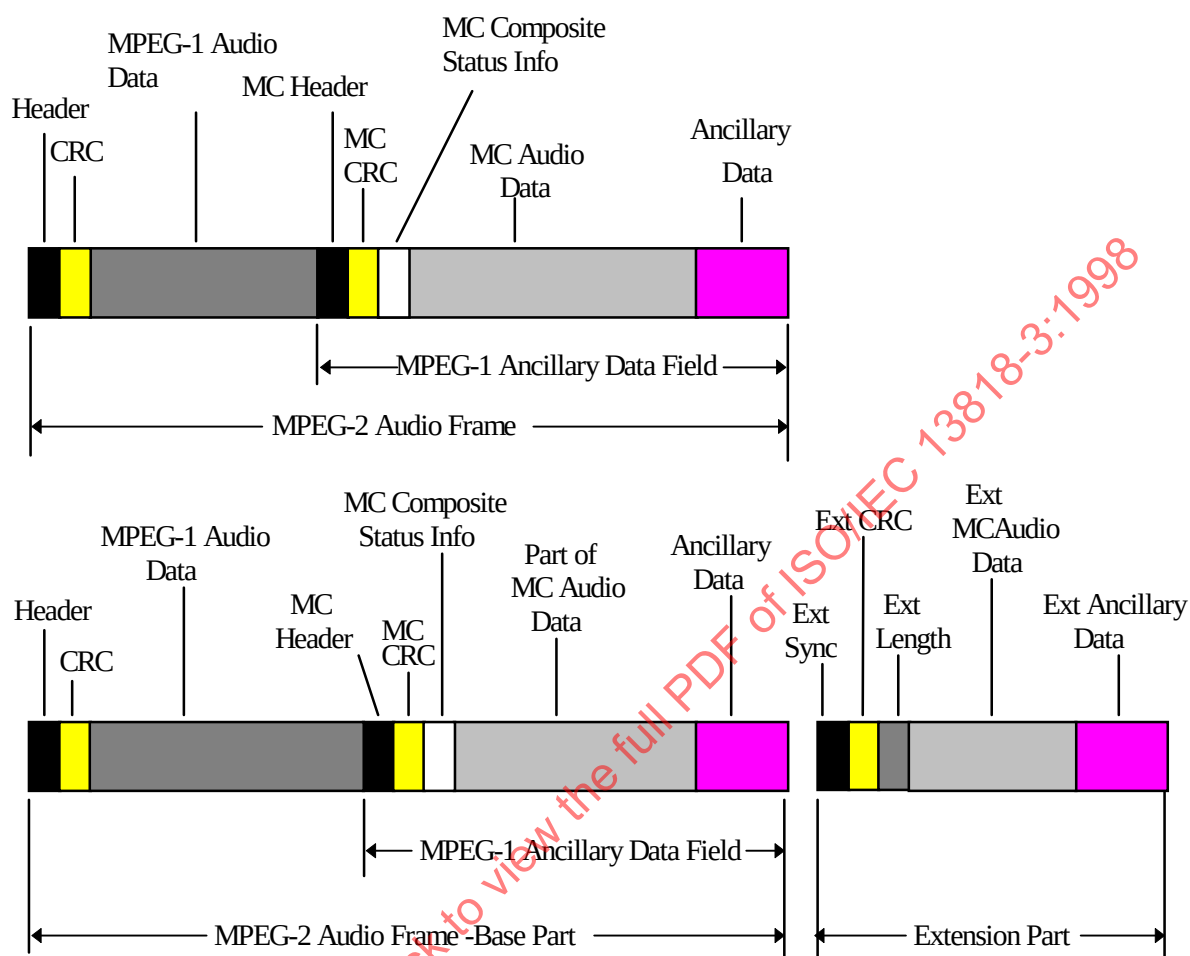
Figure A.2 — An example of a typical structure of the ISO/IEC 13818-3 Layer II multichannel extension, using the (ISO/IEC 11172-3 compatible) base bit stream, as well as the extension bit stream
