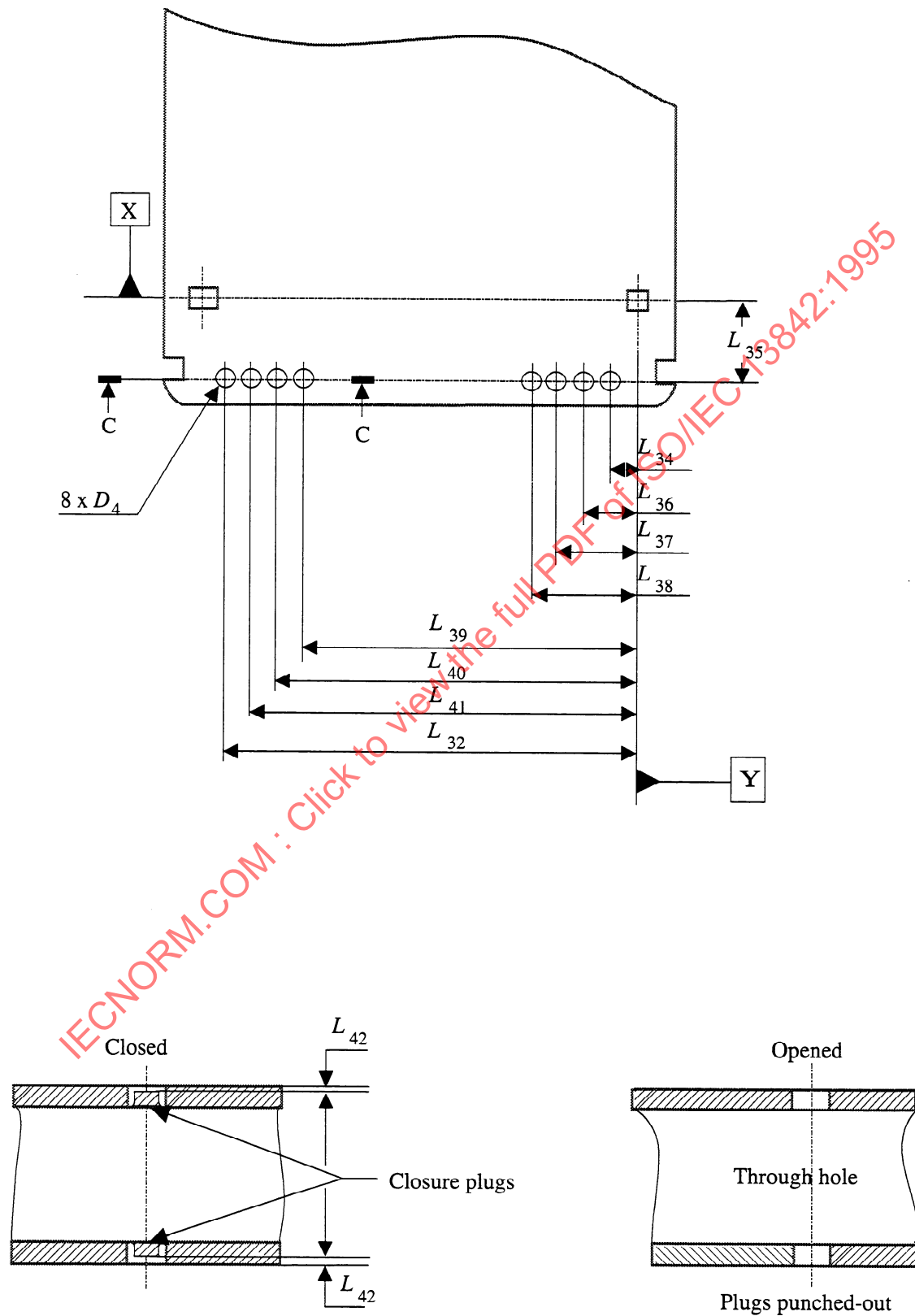
Figure 9 - Media ID sensor holes
