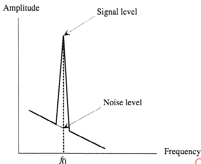
Figure 27 - Amplitude versus frequency for the magneto-optical signal
