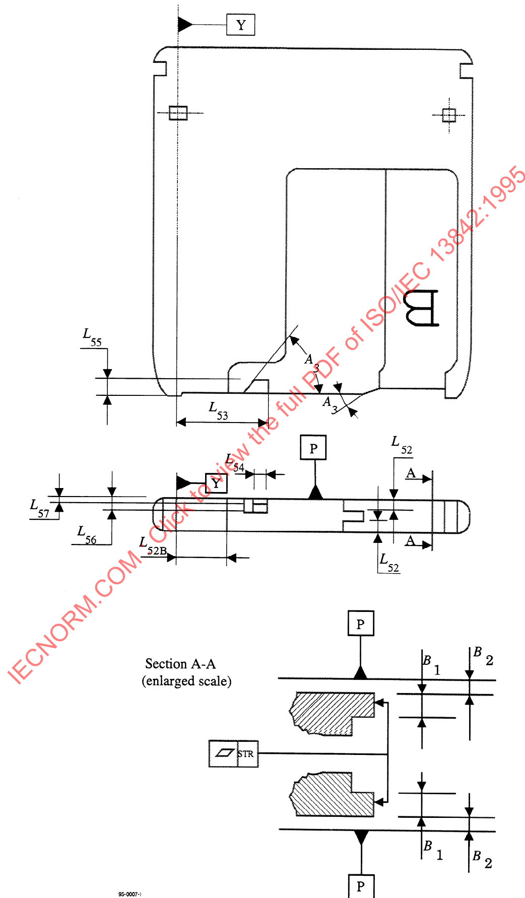
Figure 12 - Shutter opening feature
