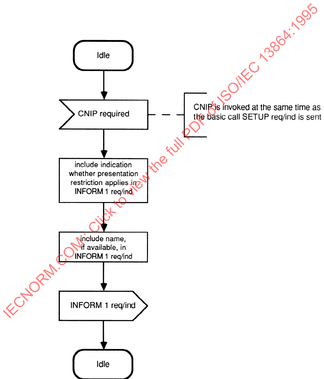
Figure 6 - SDL for Functional Entity FE1
