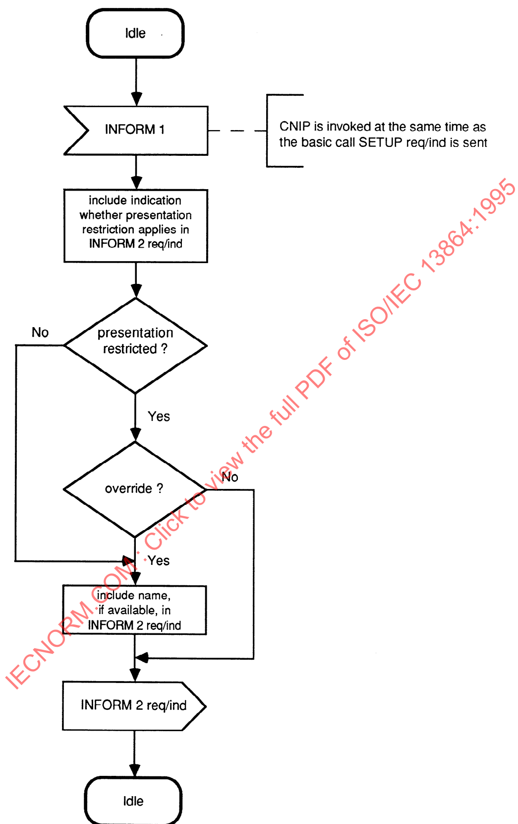
Figure 7 - SDL for Functional Entity FE2
