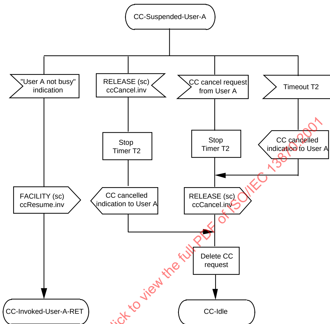
Figure D.4 — Originating PINX behaviour (continued)
