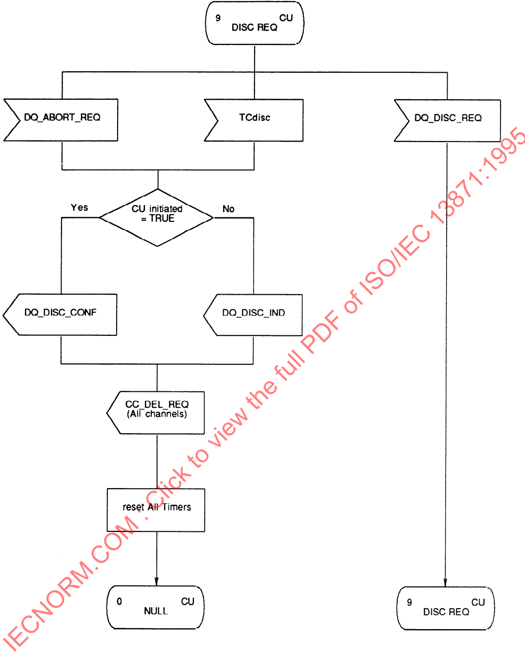
Figure D.18 - Calling Endpoint DISC REQ State
