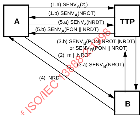
Figure 1 – Mechanism M1
