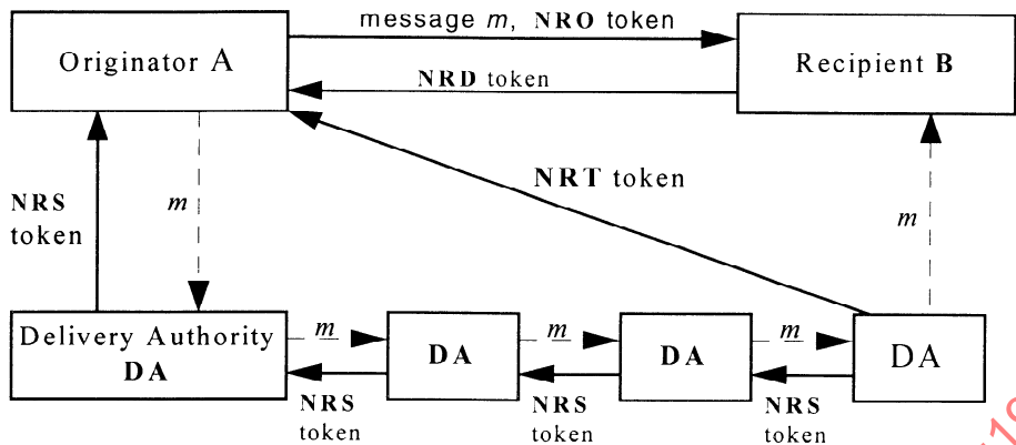
Figure 1 — Non-repudiation tokens and their usage
