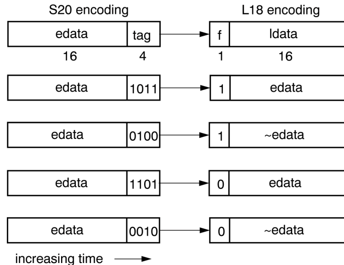
Figure 110 – S20 symbol decoding
