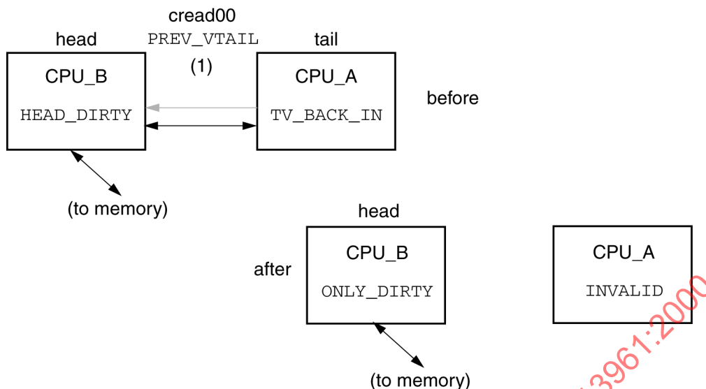
Figure 139 – Tail-entry deletions
