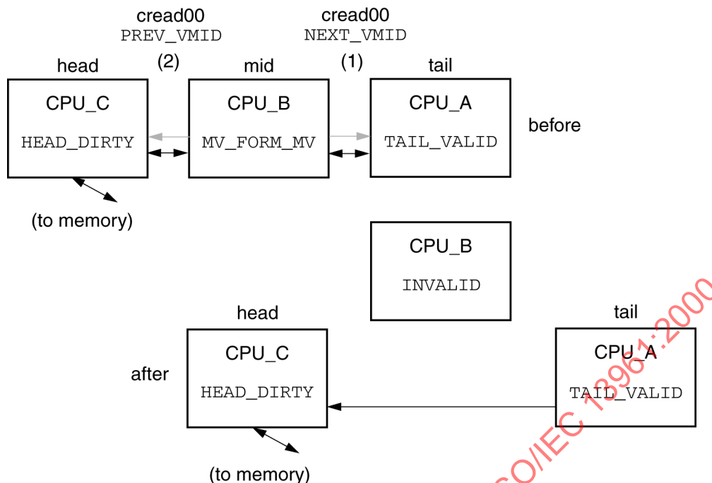
Figure 148 – Mid-entry deletions
