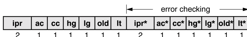
Figure 46 – Logical idle-symbol encoding
