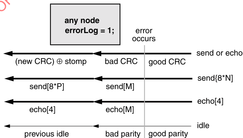
Figure 89 – Response timeouts (request and no response)
