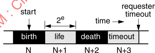
Figure 86 – Packet life-cycle intervals
