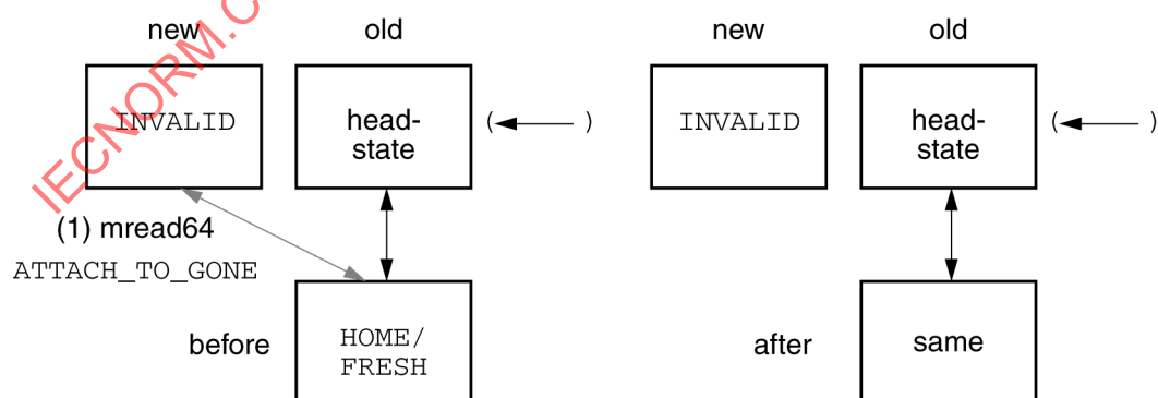
Figure 151 – Checked DMA reads
