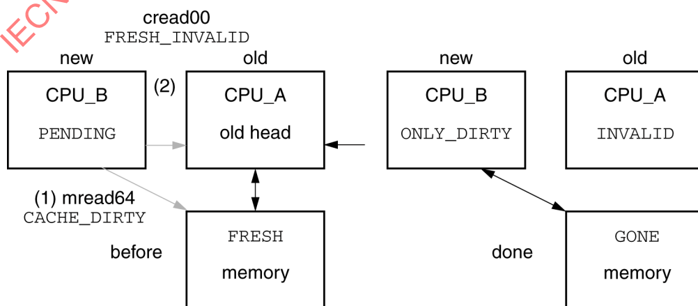
Figure 137 – FRESH list additions (minimal set)
