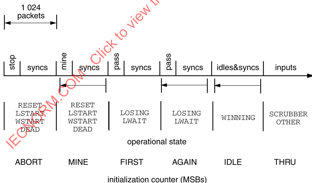
Figure 104 – Output symbol sequence during initialization
