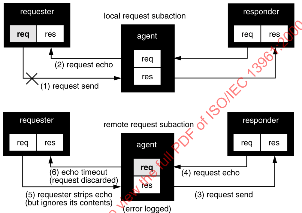
Figure 45 – Remote transaction components (local request-send damaged)
