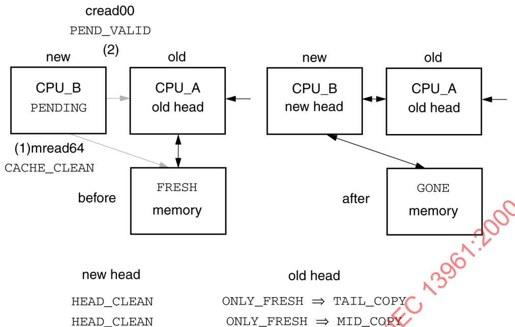
Figure 156 – CLEAN addition to FRESH list
