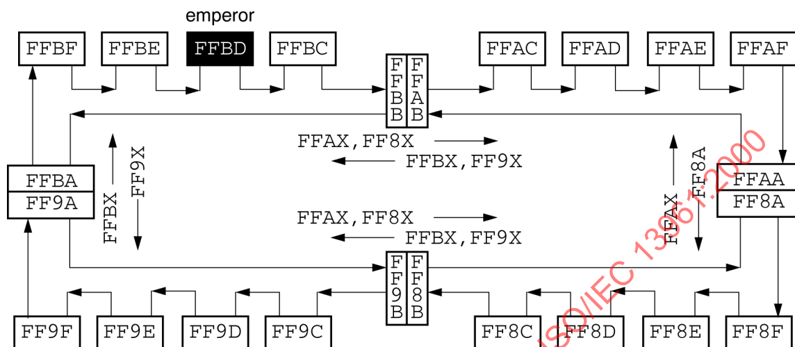
Figure 107 – Nodeids after emperor selection, final address assignments
