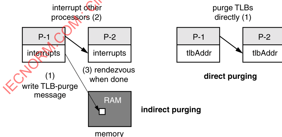
Figure 29 – TLB purging
