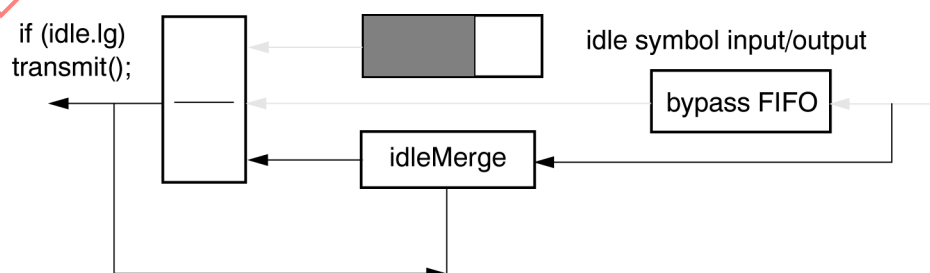
Figure 76 – Low-transmission enabled
