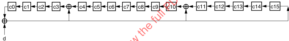
Figure 43 – Serialized implementation of 16-bit CRC
