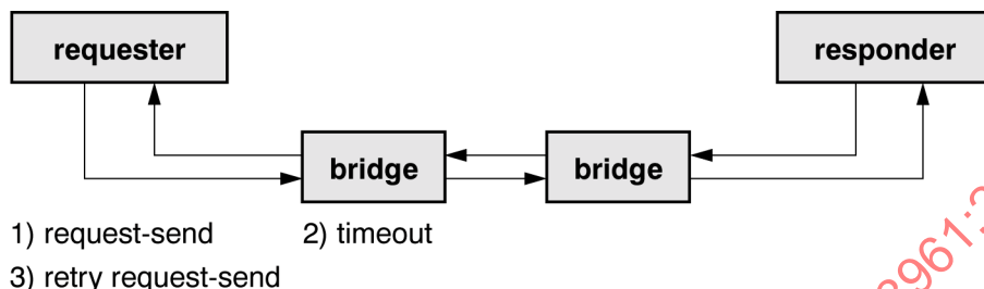
Figure 30 – Hardware fault-retry sequence
