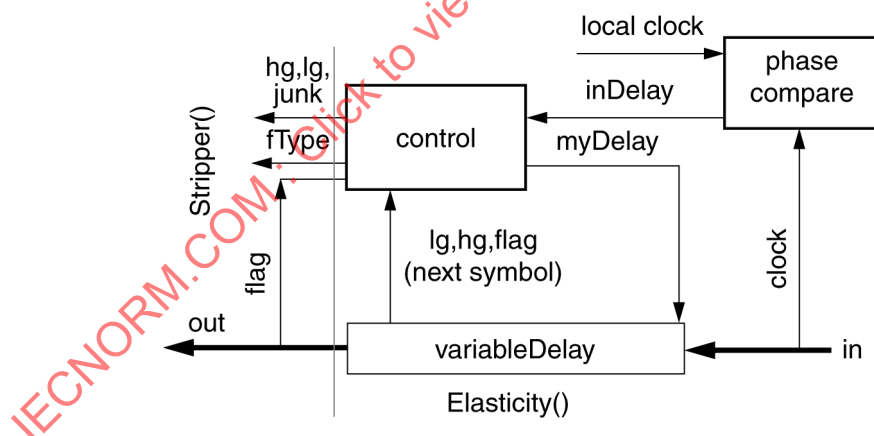
Figure 180 – Elasticity model
