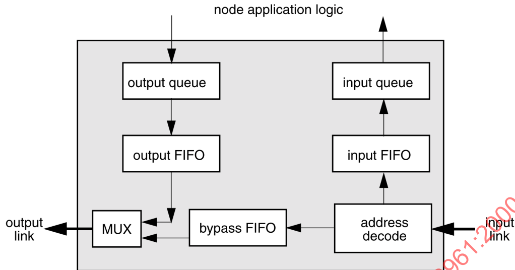
Figure 12 – Responder queues
