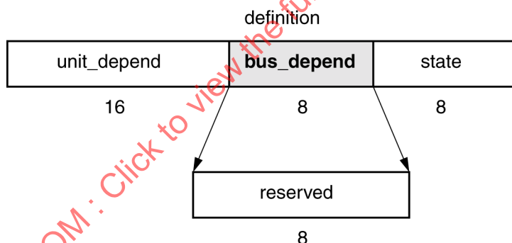
Figure 113 – STATE_CLEAR fields
