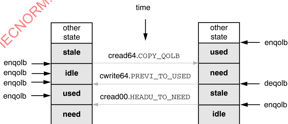
Figure 169 – QOLB usage
