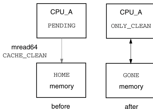
Figure 154 – CLEAN list creation
