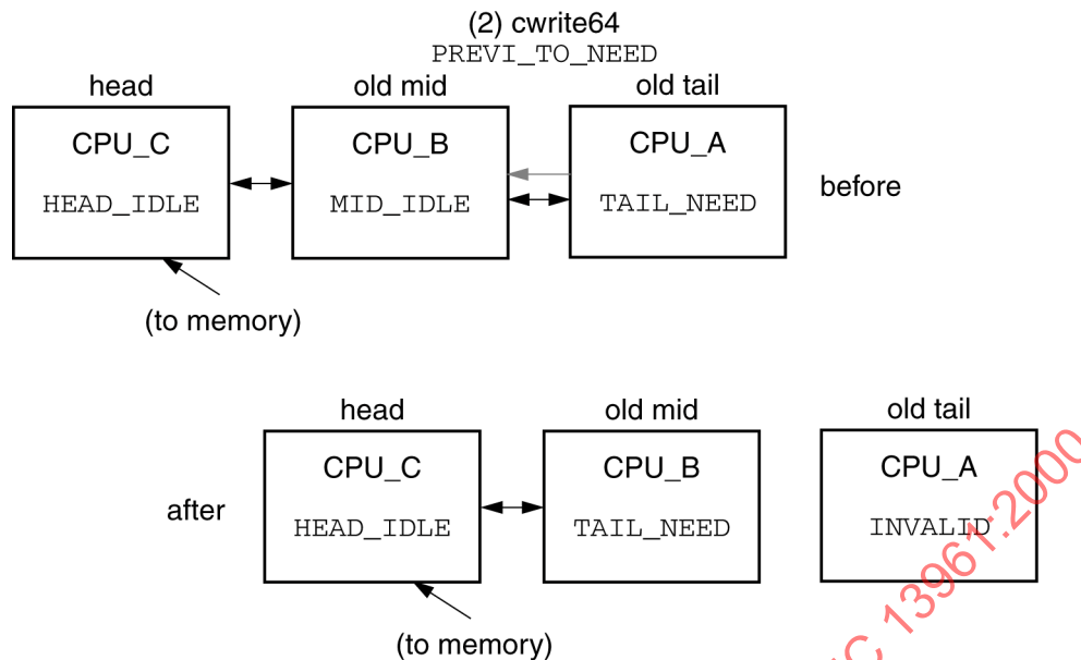
Figure 168 – Deqolb tail-deletion on QOLB sharing list
