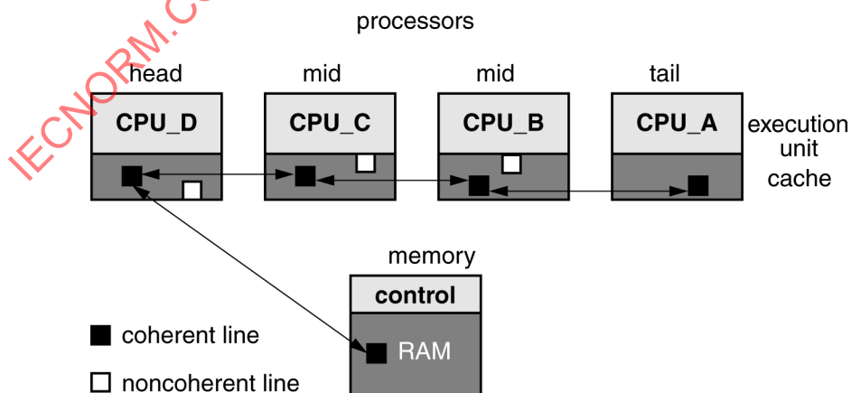
Figure 26 – Distributed cache tags
