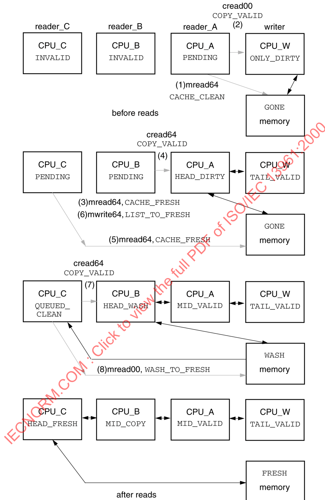
Figure 158 – Washing DIRTY sharing lists (prepend conflict)
