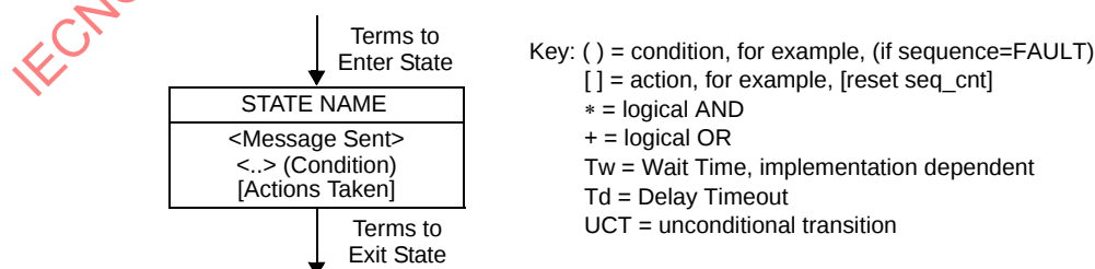
Figure 1 – State diagram notation example
