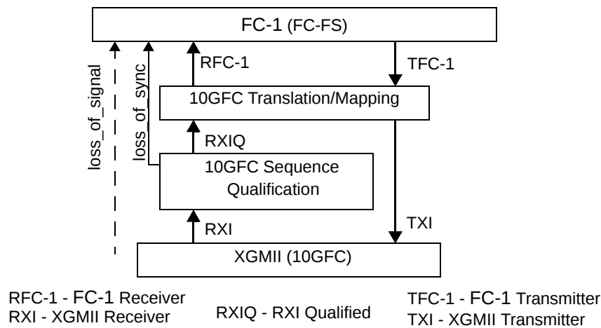
Figure 12 – FC-1/10GFC/XGMII Interaction
