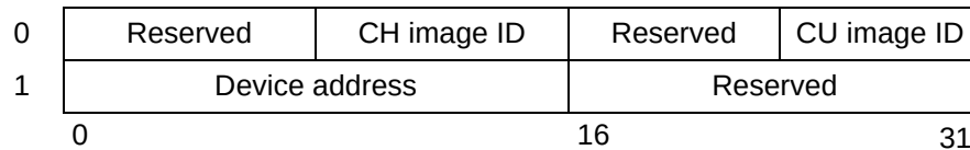
Figure 13 – SB-2 header
