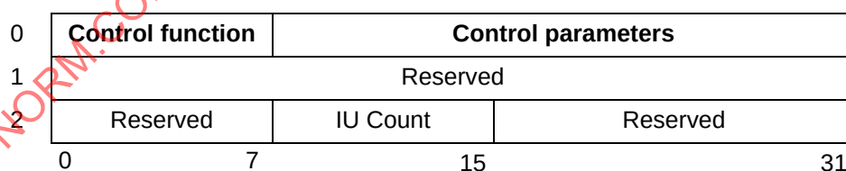
Figure 31 – Control header
