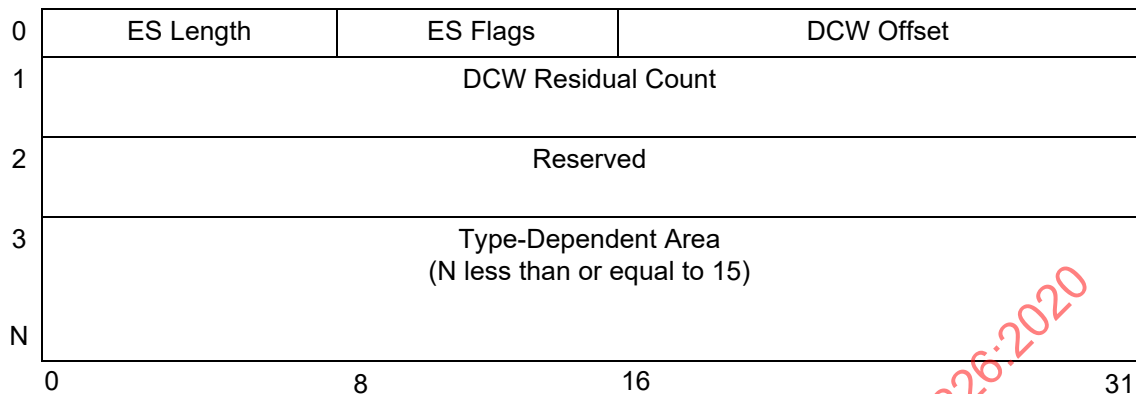
Figure 57 – Extended Status General Format
