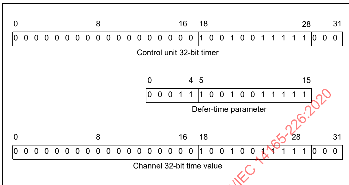
Figure 35 – Defer-Time Parameter Example
