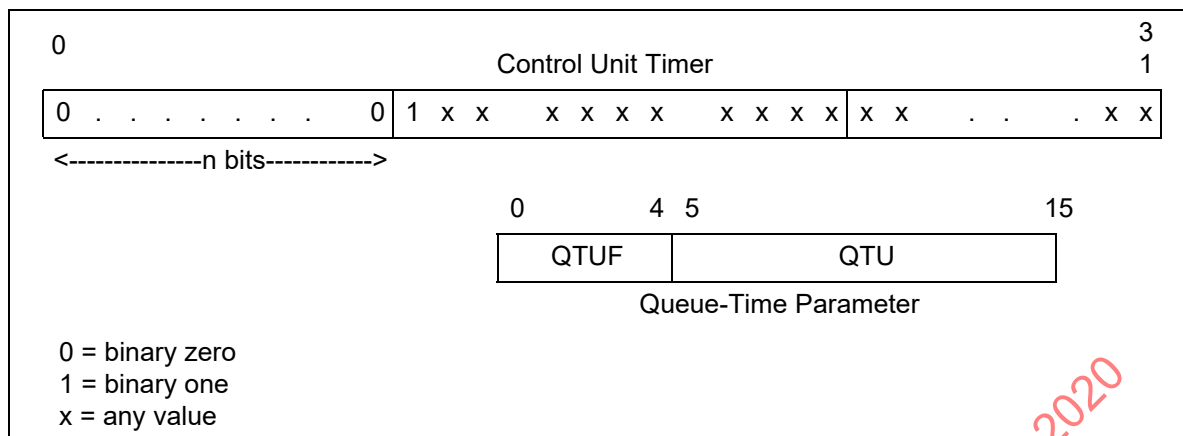
Figure 32 – Queue-Time Parameter (QTP) Format
