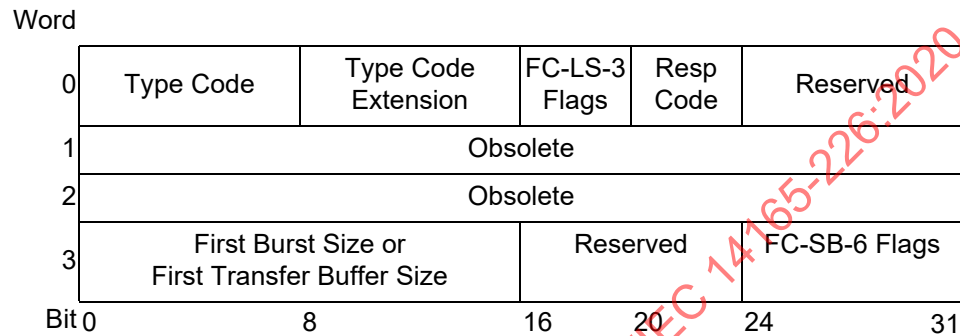
Figure 12 – Service Parameter Response Page for a PRLI LS_ACC
