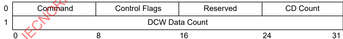
Figure 47 – Device Command Word
