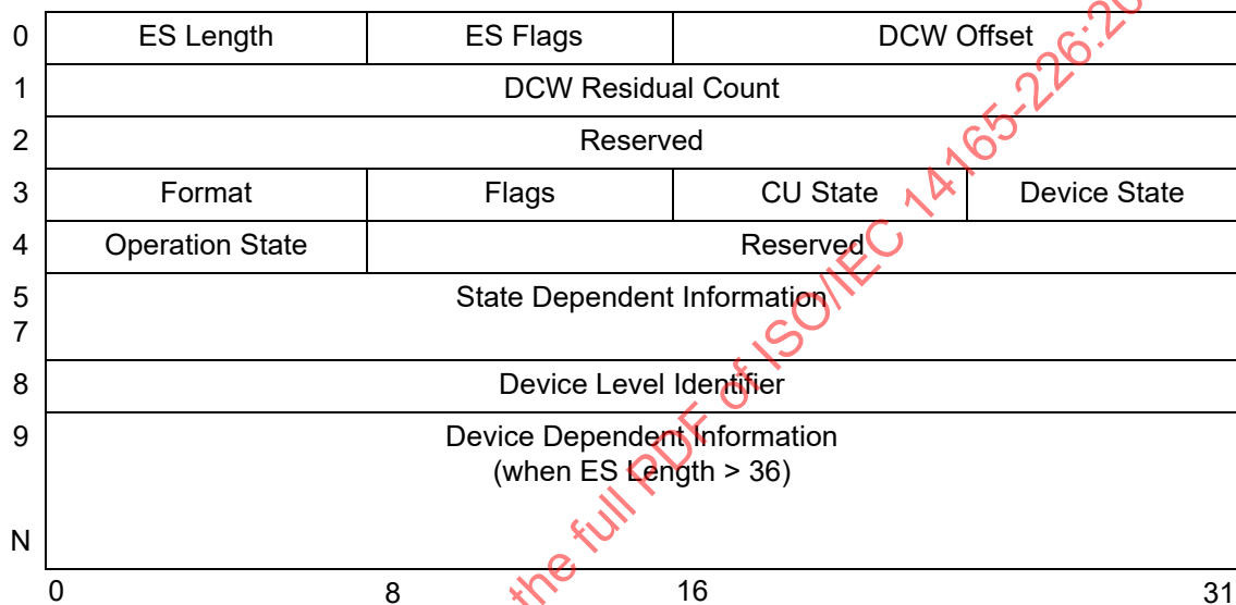
Figure 61 – Interrogate Extended Status Format
