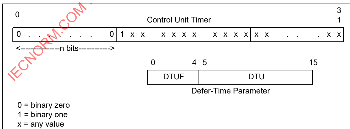
Figure 34 – Defer Time Parameter Format
