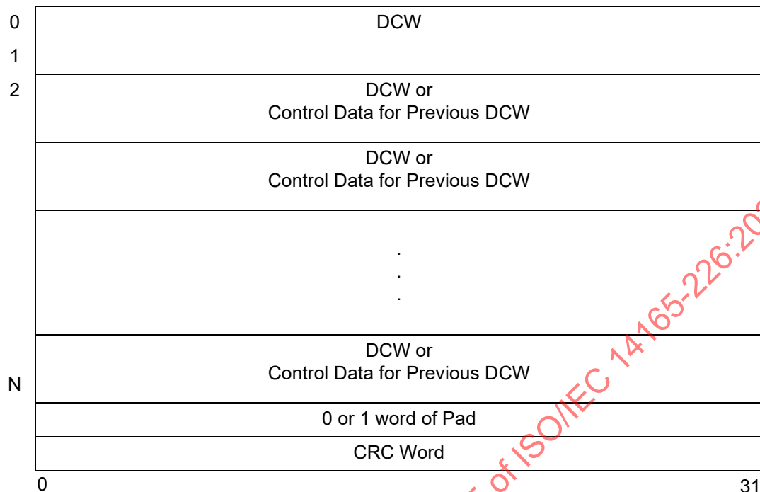
Figure 50 – Transport-Command Area Extended (TCAX) plus Pad Bytes and CRC
