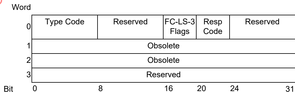
Figure 14 – Logout Parameter Page for a PRLO LS_ACC
