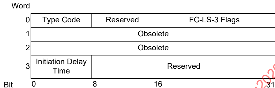
Figure 13 – Logout Parameter Page for a PRLO request
