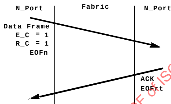
Figure 50 - Class 4 circuit - CTI or CTR initiated removal
