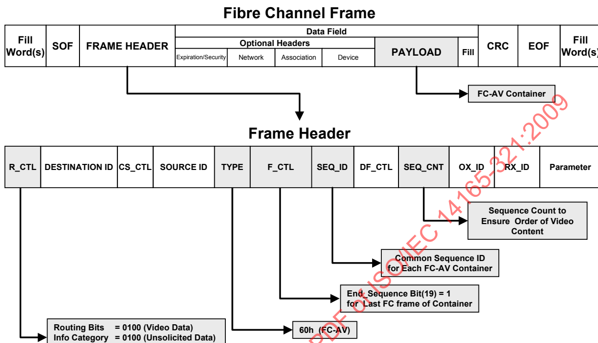
Figure 14 – FHCP Frame Header
