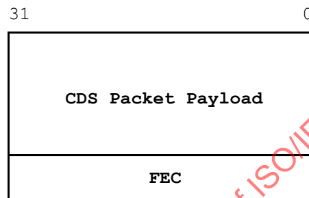
Figure 9 – CDS Packet Format
