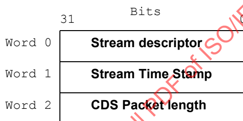
Figure 5 – Stream Header format
