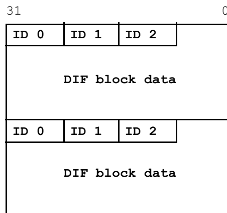
Figure 10 – CDS Packet Payload format (SMPTE)
