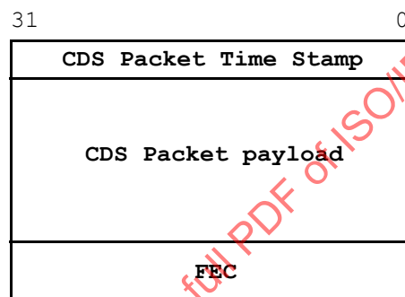
Figure 12 – CDS Packet format (MPEG-TS)
