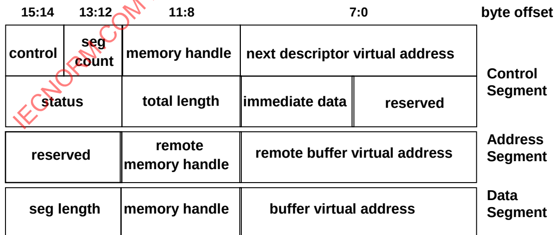
Figure 5: RDMA Descriptor Format
