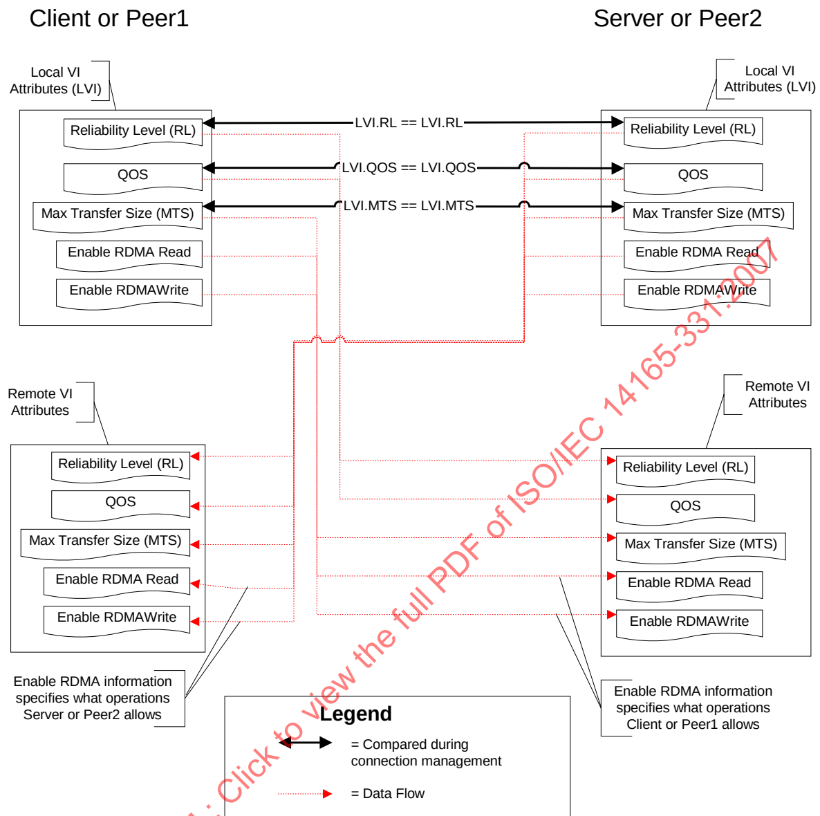
Figure 13: VI Attribute Comparison and Exchange
