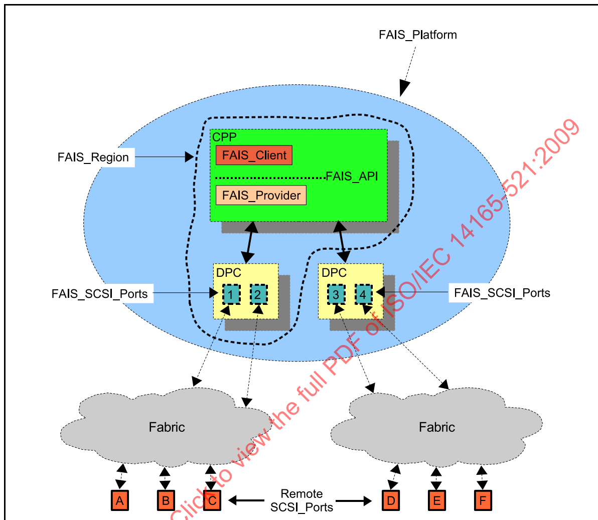
Figure 5 – Operational layering
