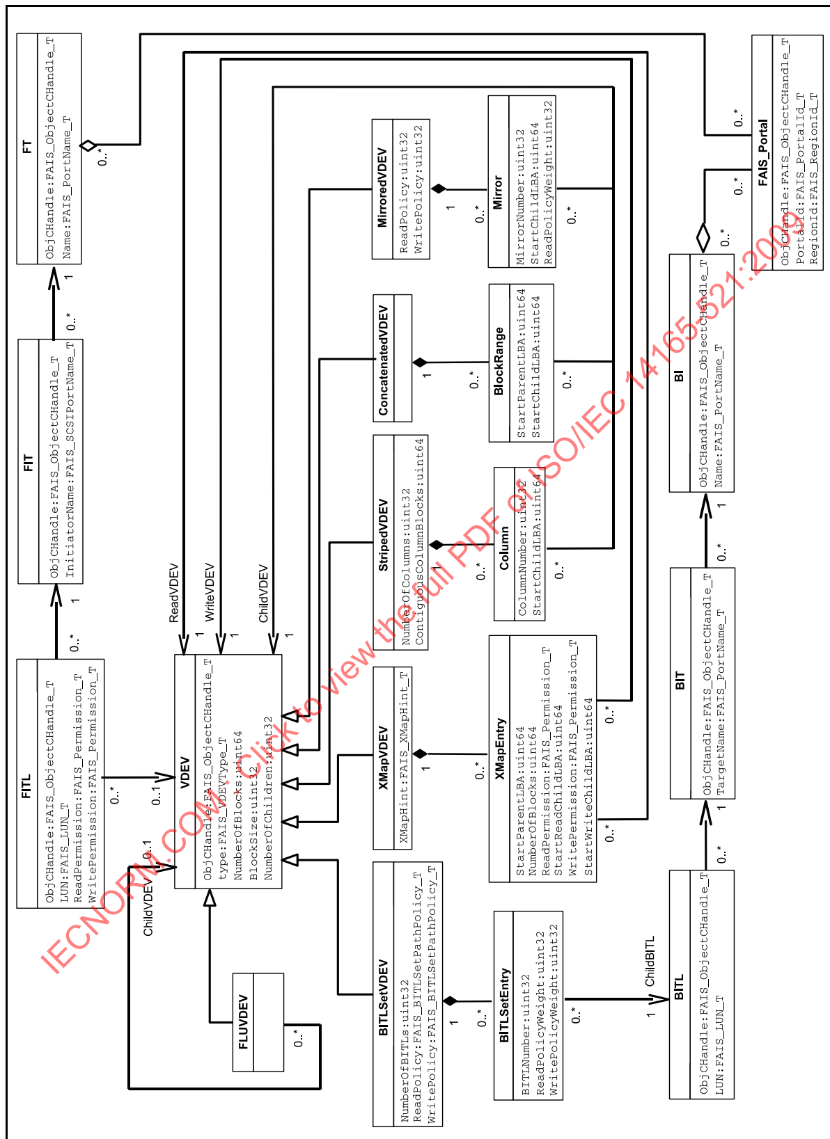
Figure 6 – Object model
