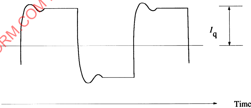
Figure 1 - Quiescent value of the Test Recording Current
