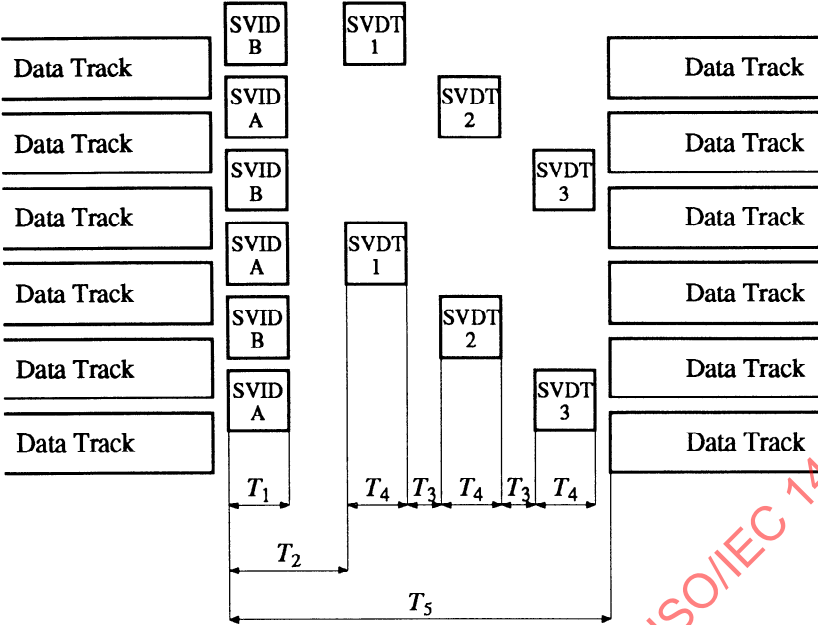
Figure 10 - Layout of the Servo Sector
