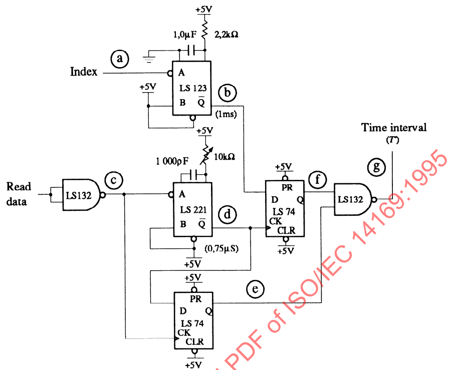
Figure F.1 - Measurement Circuit
