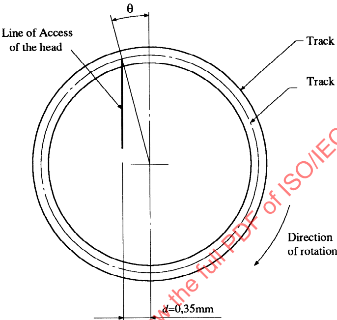
Figure 2 - Recording offset angle, seen on Side 1
