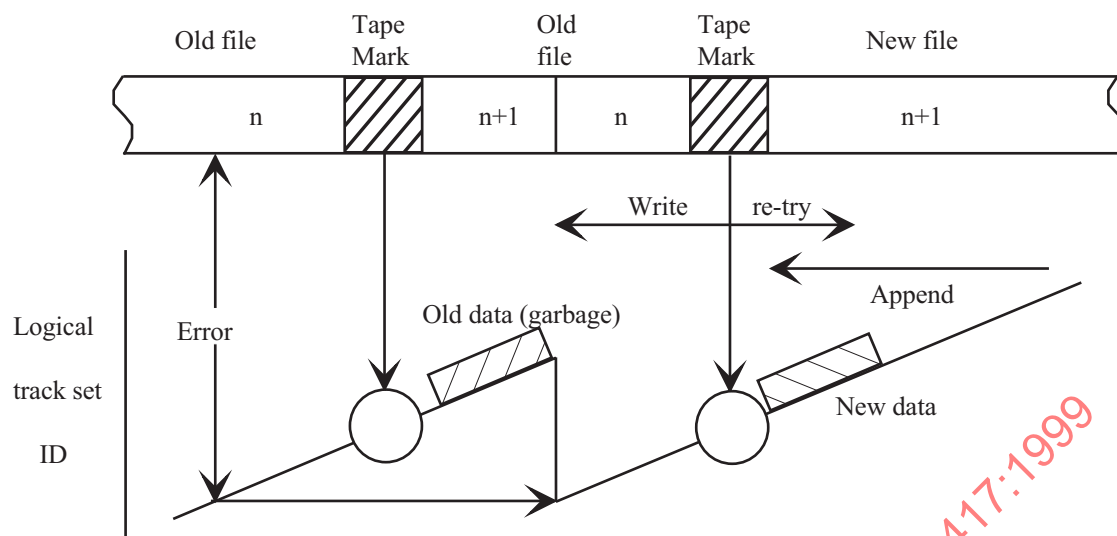
Figure C.3 - Appending file over re-tried area without track set ID offset
