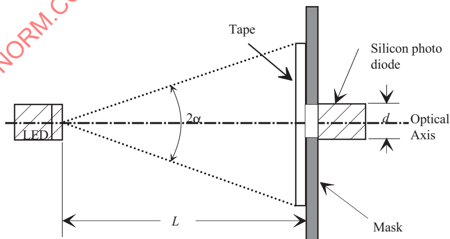
Figure A.1 - Optical arrangement
