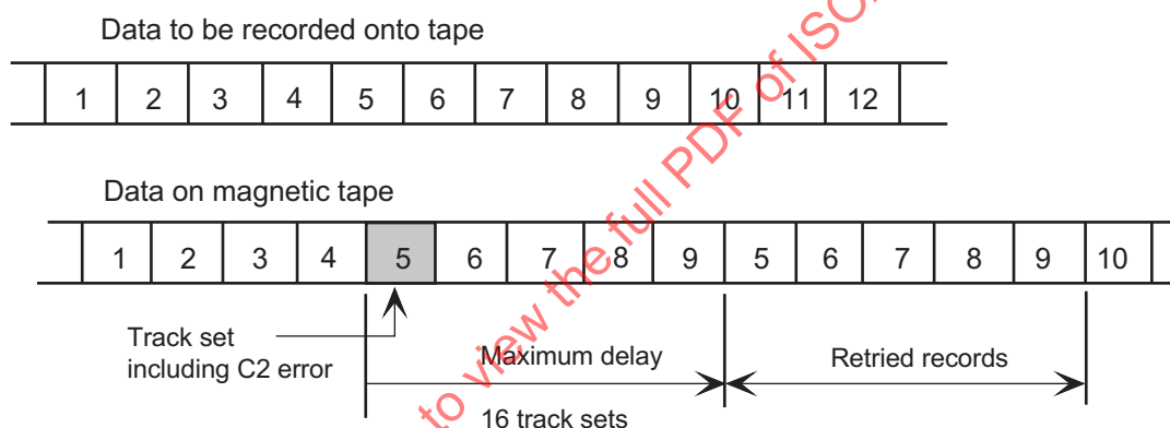
Figure 21 - Example of write retry sequence
