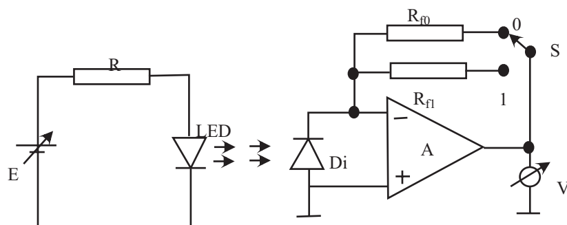
Figure A.2 - Measuring circuitry
