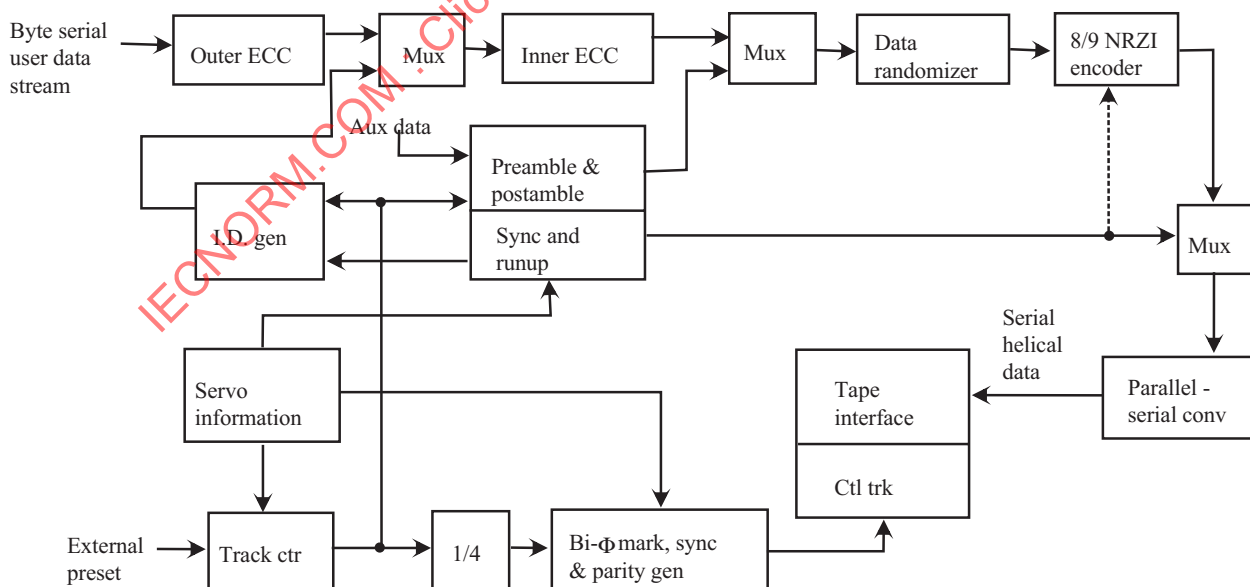
Figure 11 - Digital recorder: conceptual block diagram of record path
