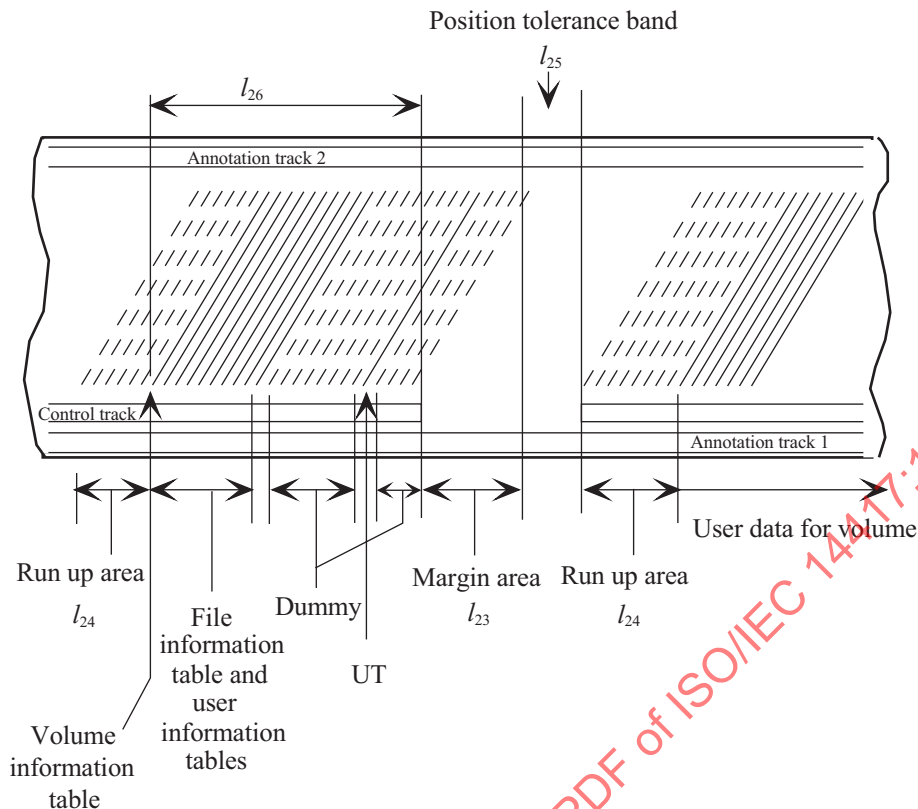
Figure 20 - Allocation of DIT
