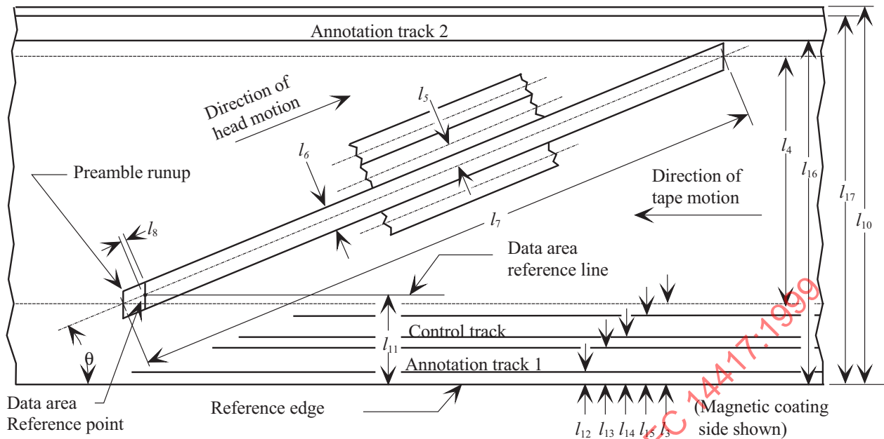
Figure 13 - Location and dimensions of recorded tracks
