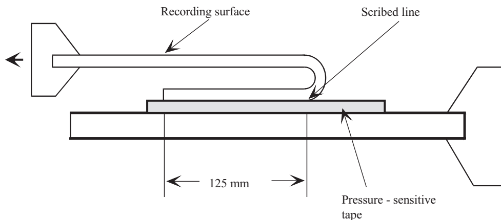
Figure 3 - Measurement of coating adhesion
