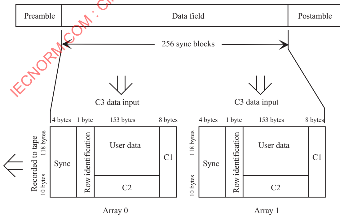
Figure 9 - C1 and C2 ECC
