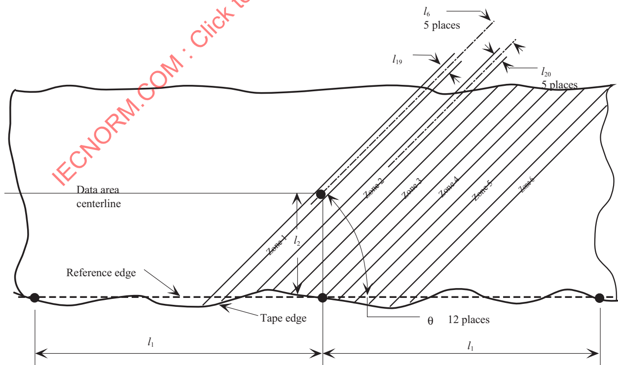
Figure 14 - Location and dimensions of tolerance zones for helical tracks
