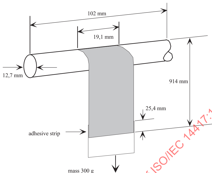
Figure 2 - Measurement of layer-to-layer adhesion
