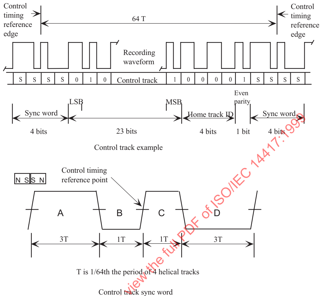
Figure 16 Recorded control track waveform timing
