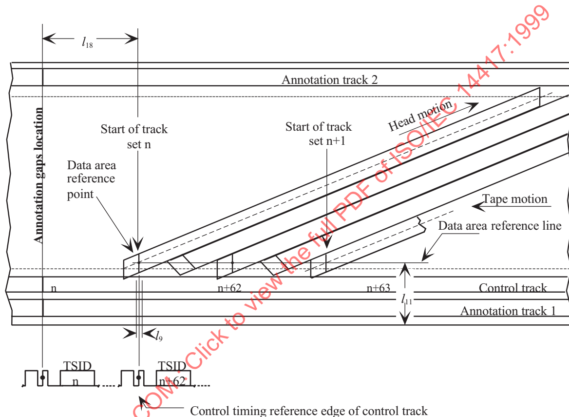
Figure 15 - Location of longitudinal tracks and 32 bit control word
