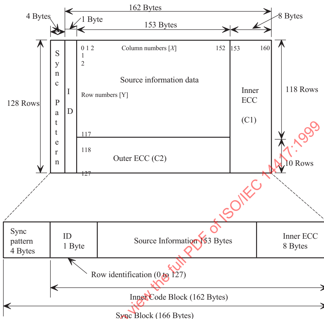
Figure 10 - Sync block
