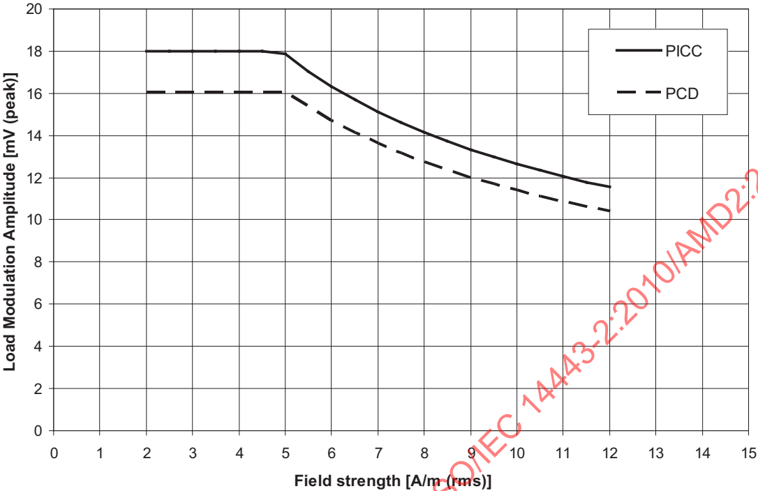
Figure 13 — Load modulation amplitude limits for “Class 4”
