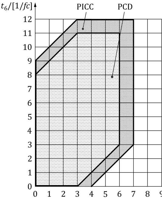
Figure 7 — PauseA timing parameters for a bit rate of fc/64
