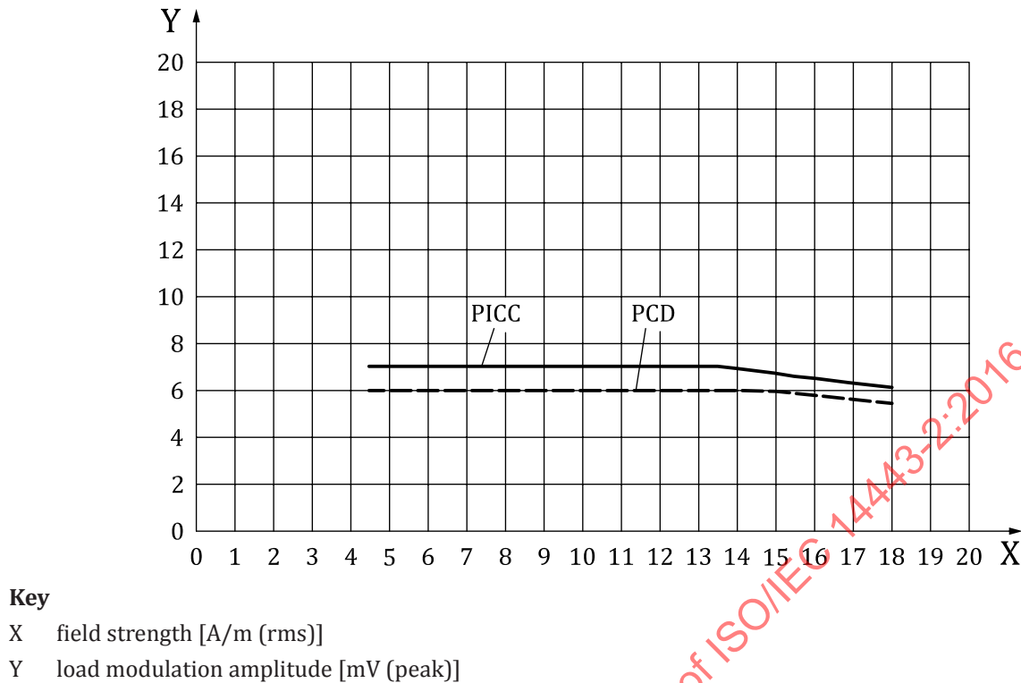
Figure 15 — Load modulation amplitude limits for “Class 6”
