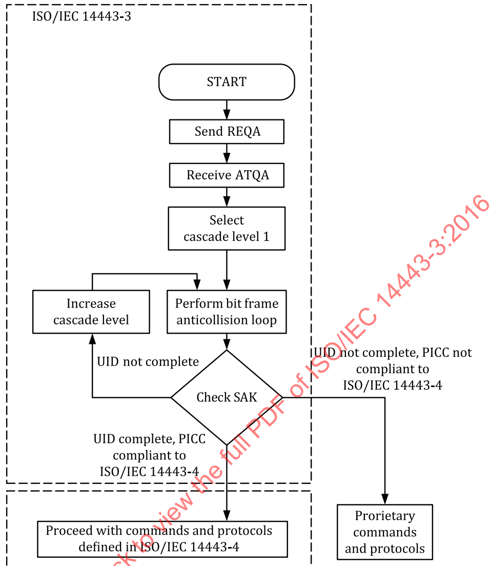
Figure 9 — Initialization and anticollision flowchart for PCD
