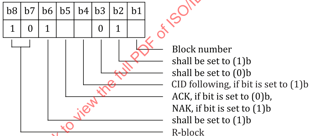
Figure 17 — Coding of R-block PCB
