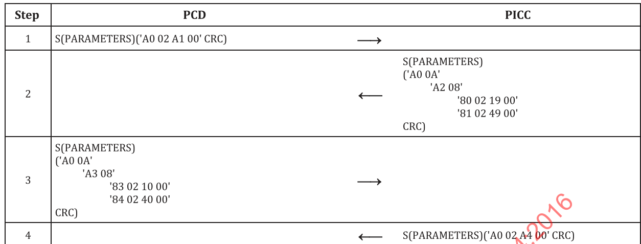
Figure 26 — Bit rates activation example
