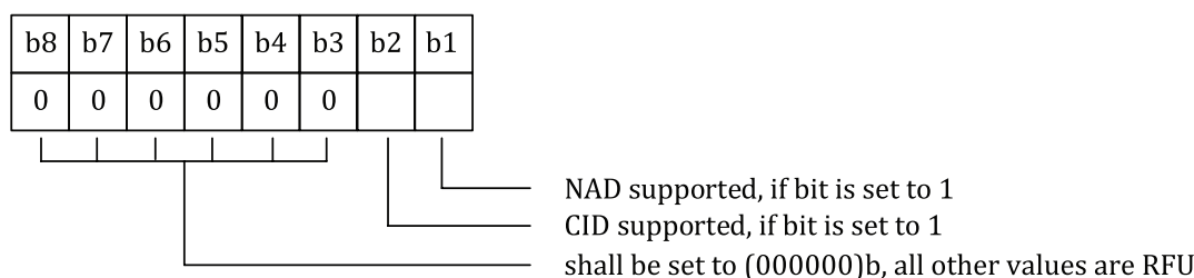
Figure 8 — Coding of interface byte TC(1)
