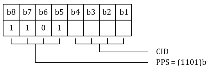
Figure 10 — Coding of PPSS
