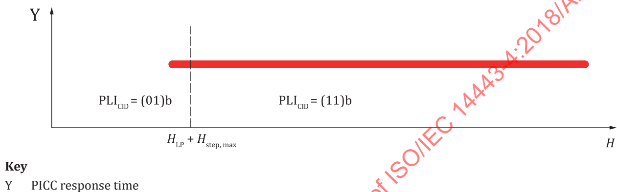
Figure H.1 — PICC response time not depending on field strength
