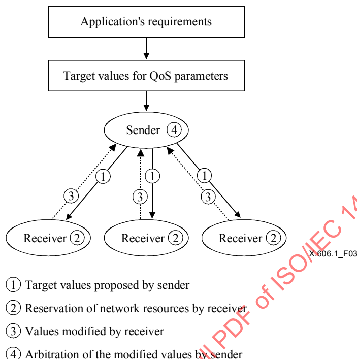
Figure 3 – QoS negotiation
