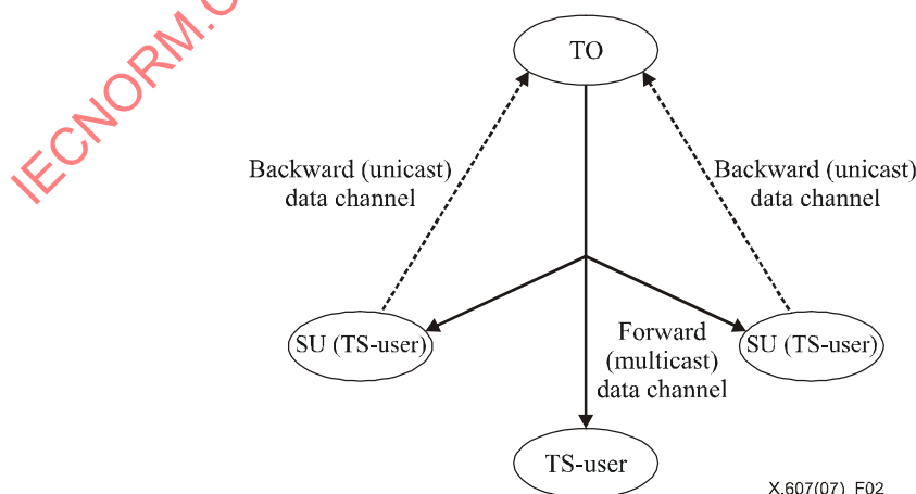
Figure 2 – Data transport in ECTP-3
