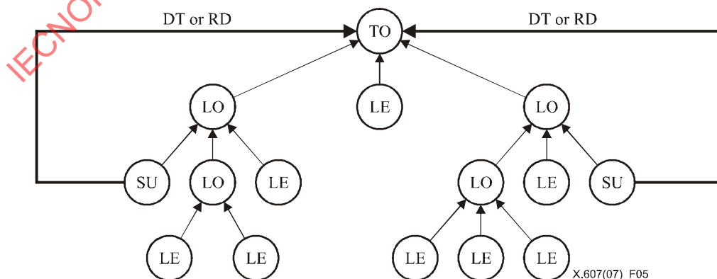
Figure 5 – Backward data channels in ECTP-3
