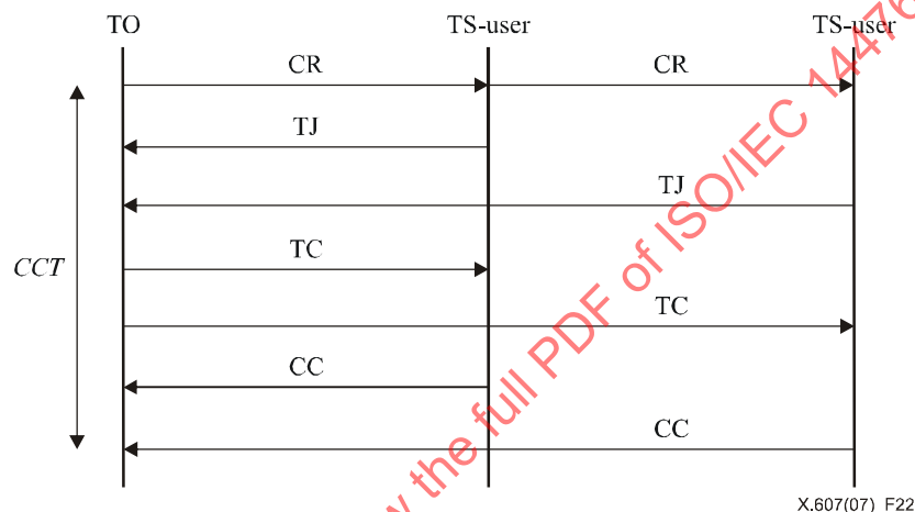
Figure 22 – Connection Creation procedures
