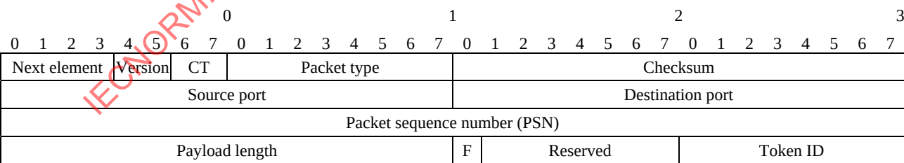
Figure 8 – Base header (ECTP over IP)
