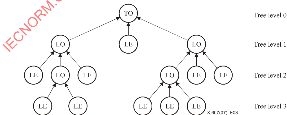
Figure 3 – Control tree in ECTP-3
