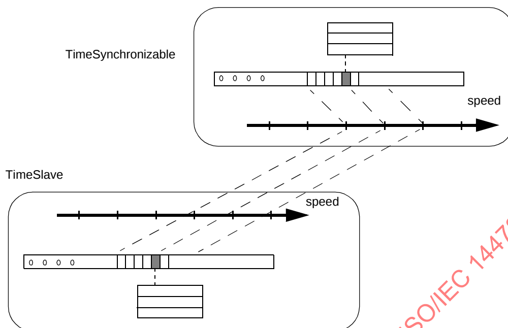
Figure 7 — TimeSlave object
