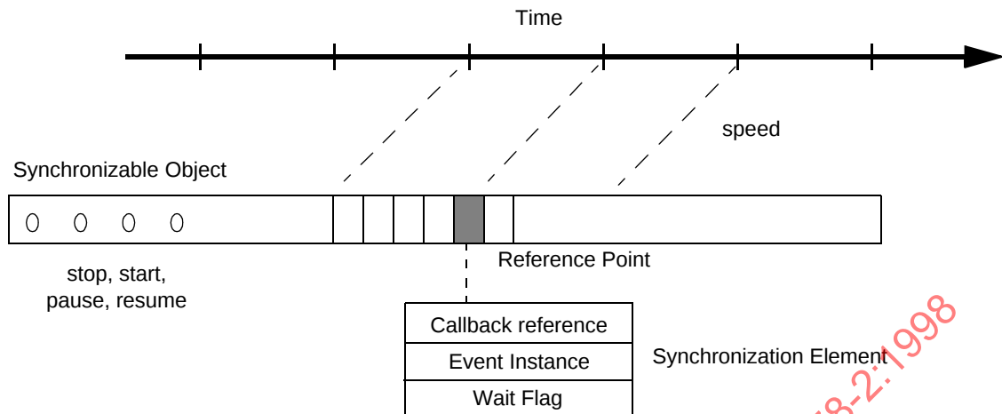
Figure 6 — TimeSynchronizable object
