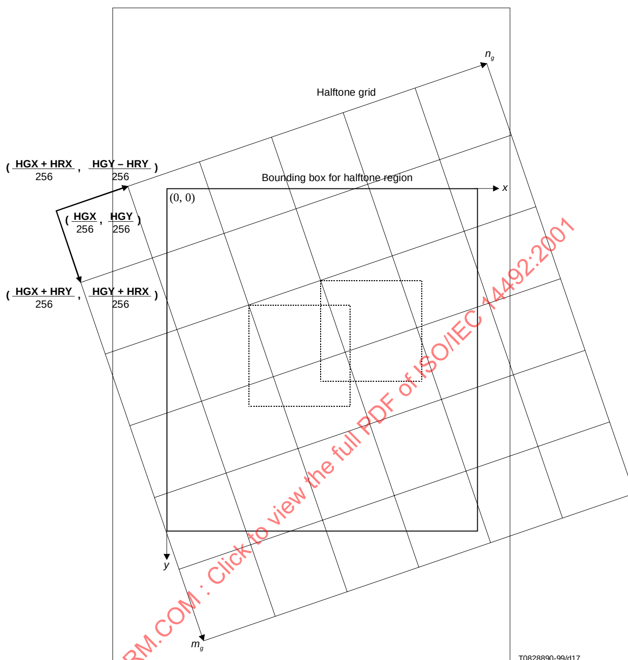
Figure 24 – Specification of coordinate systems and grid parameters
