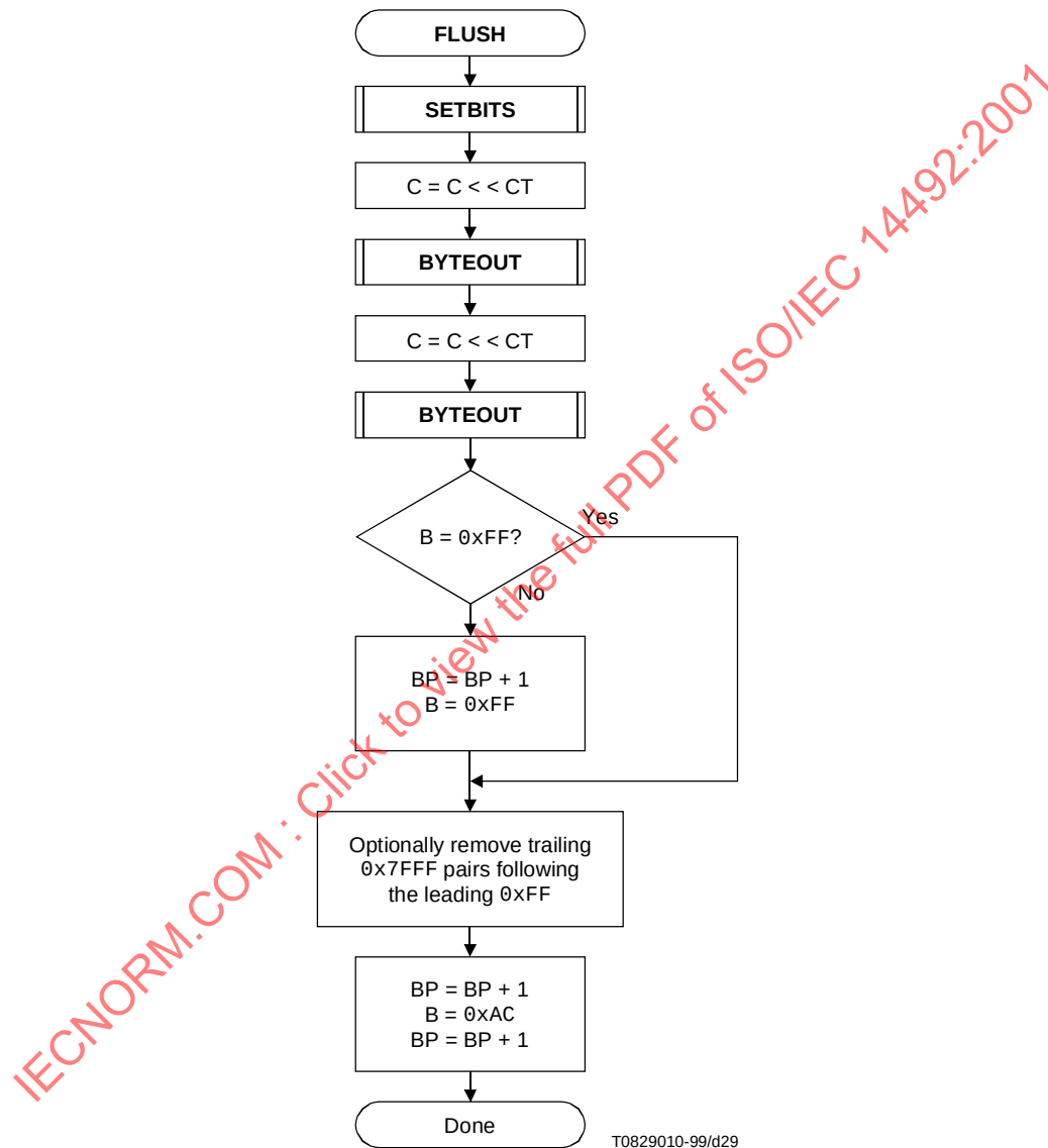
Figure E.11 – FLUSH procedure
