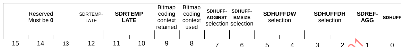
Figure 31 – Symbol dictionary flags field structure
