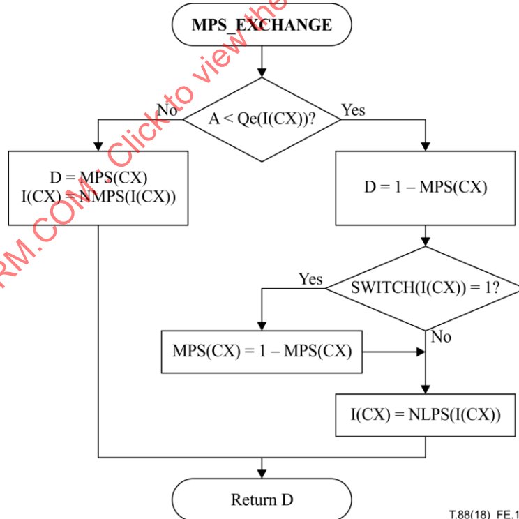
Figure E.16 – Decoder MPS path conditional exchange procedure
