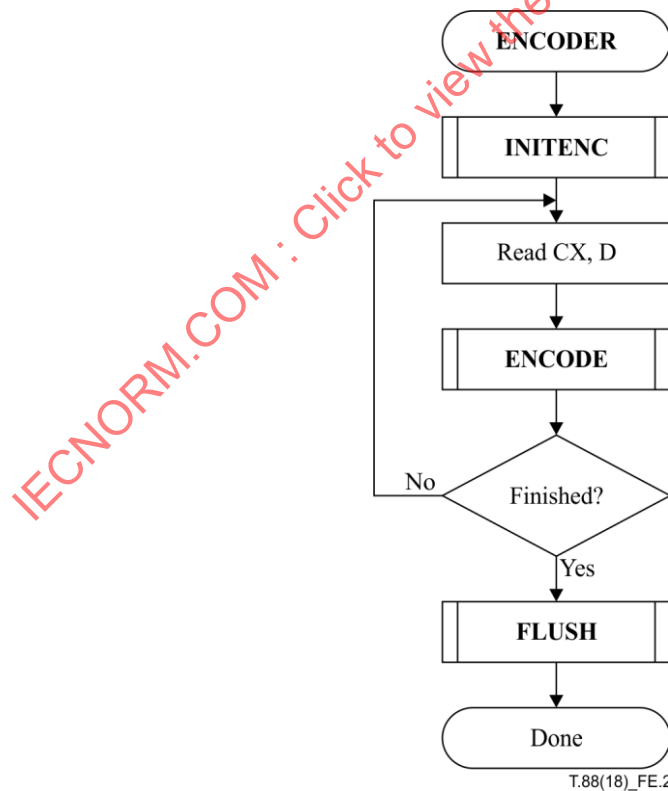
Figure E.2 – Encoder for the MQ-coder
