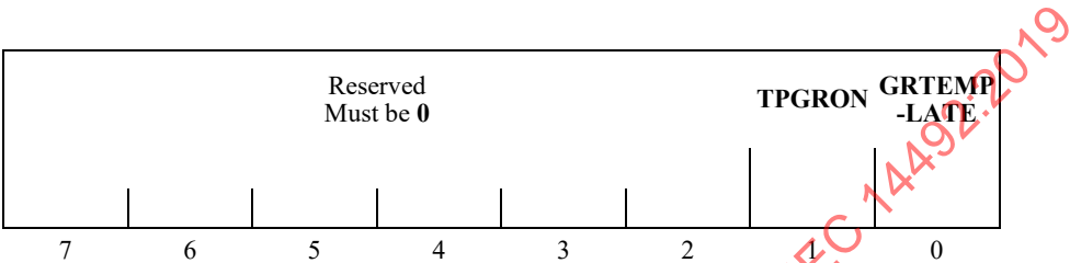
Figure 53 – Generic refinement region segment flags field structure
