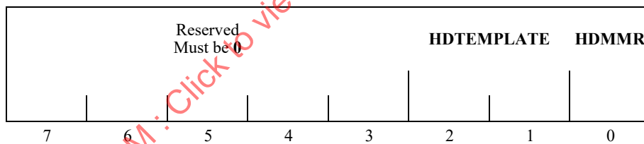
Figure 42 – Pattern dictionary flags field structure
