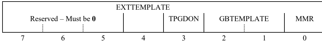
Figure 48 – Generic region segment flags field structure
