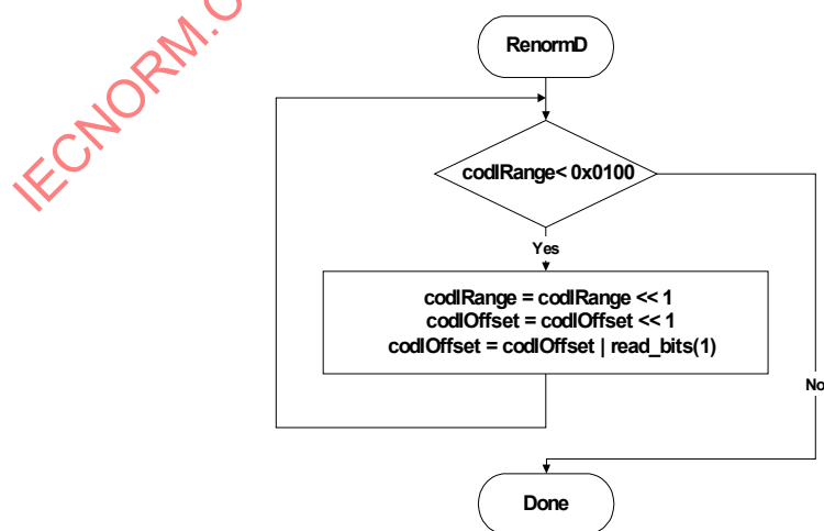
Figure 9-4 – Flowchart of renormalization
