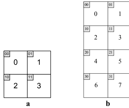
Figure 8-7 – Assignment of the indices of dcC to chroma4x4BlkIdx: (a) ChromaArrayType equal to 1, (b) ChromaArrayType equal to 2
