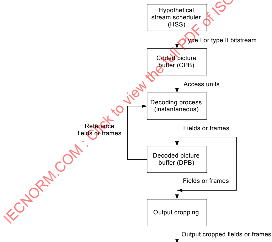
Figure C-2 – HRD buffer model
