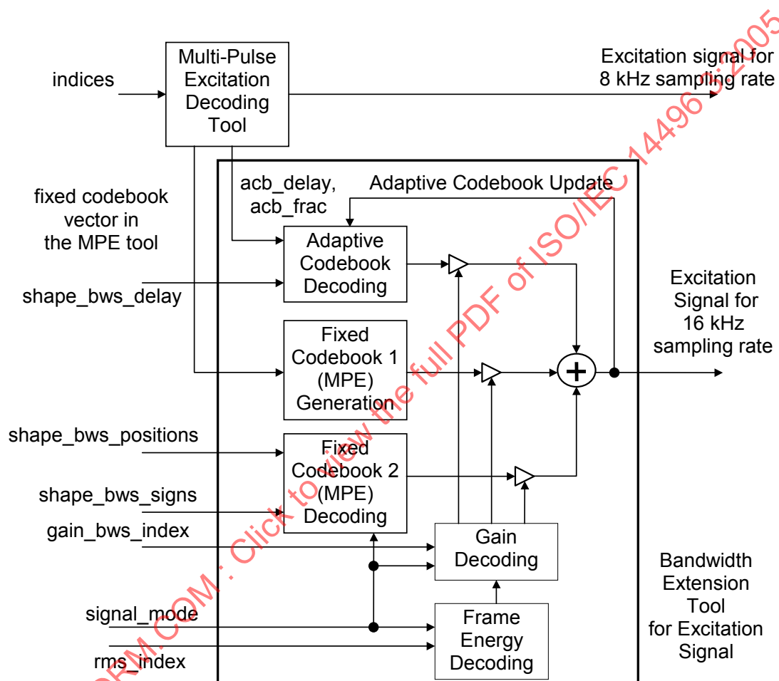
Figure 3.9 — Bandwidth scalable multi-pulse excitation generation process
