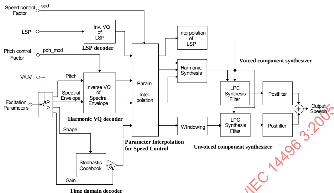
Figure 2.2 — Block diagram of the HVXC decoder
