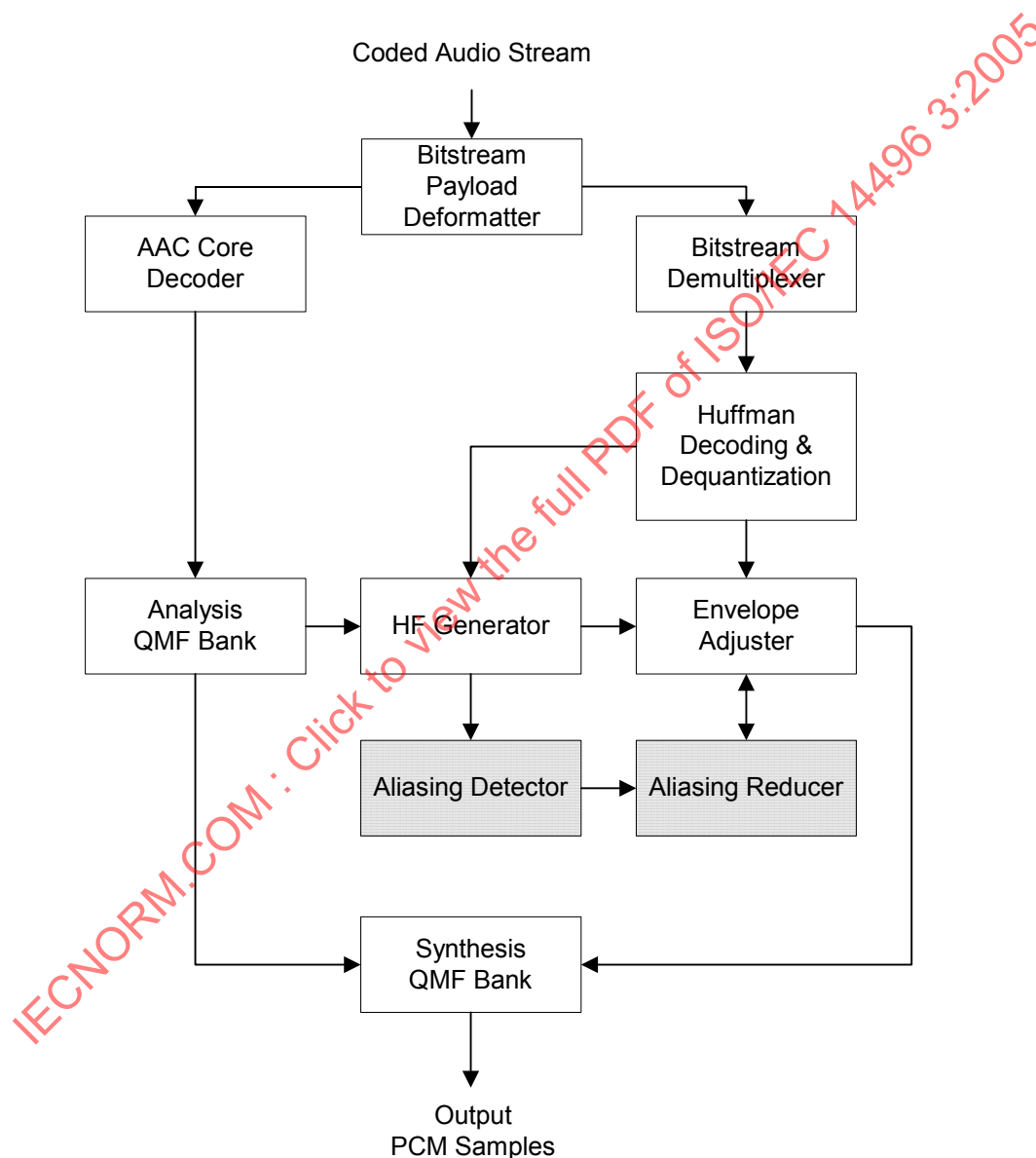
Figure 4.47 – Block diagram of the SBR low power decoder
