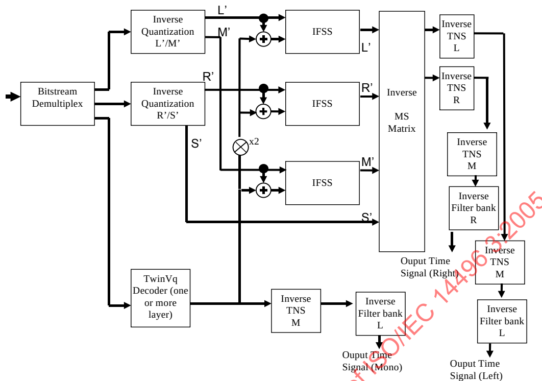
Figure 4.15 – Decoding of a TwinVQ (mono) + AAC (stereo) configuration, if TNS is used in the first TwinVQ layer
