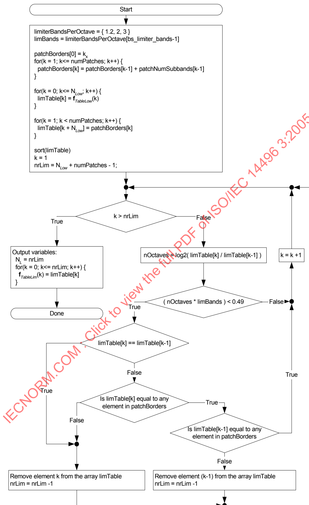
Figure 4.40 – Calculation of f_{TableLim} if bs\_limiter\_bands > 0
