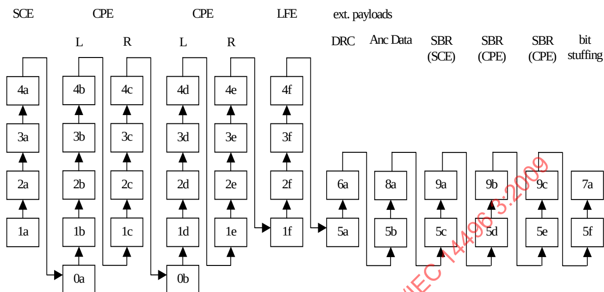
Figure 4.25 – Dependency structure in the case of error resilient multichannel AAC syntax ( \text{channelConfiguration} == 6 )
