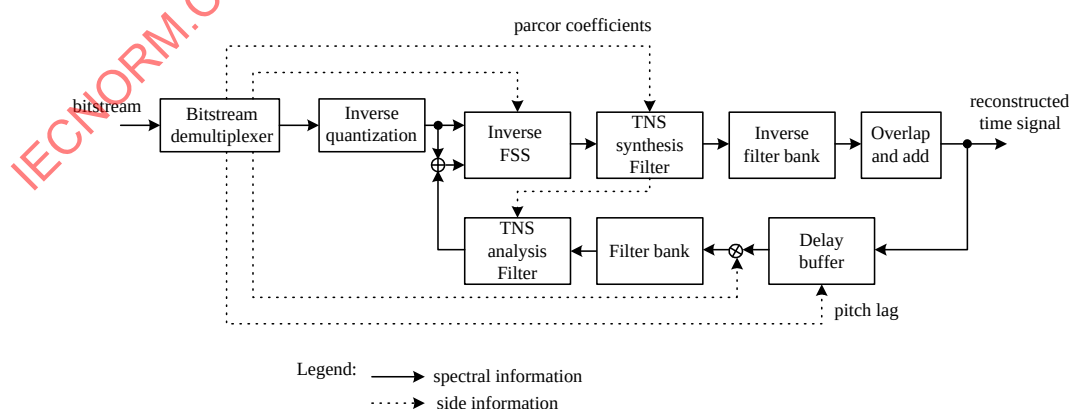
Figure 4.37 – Decoder structure
